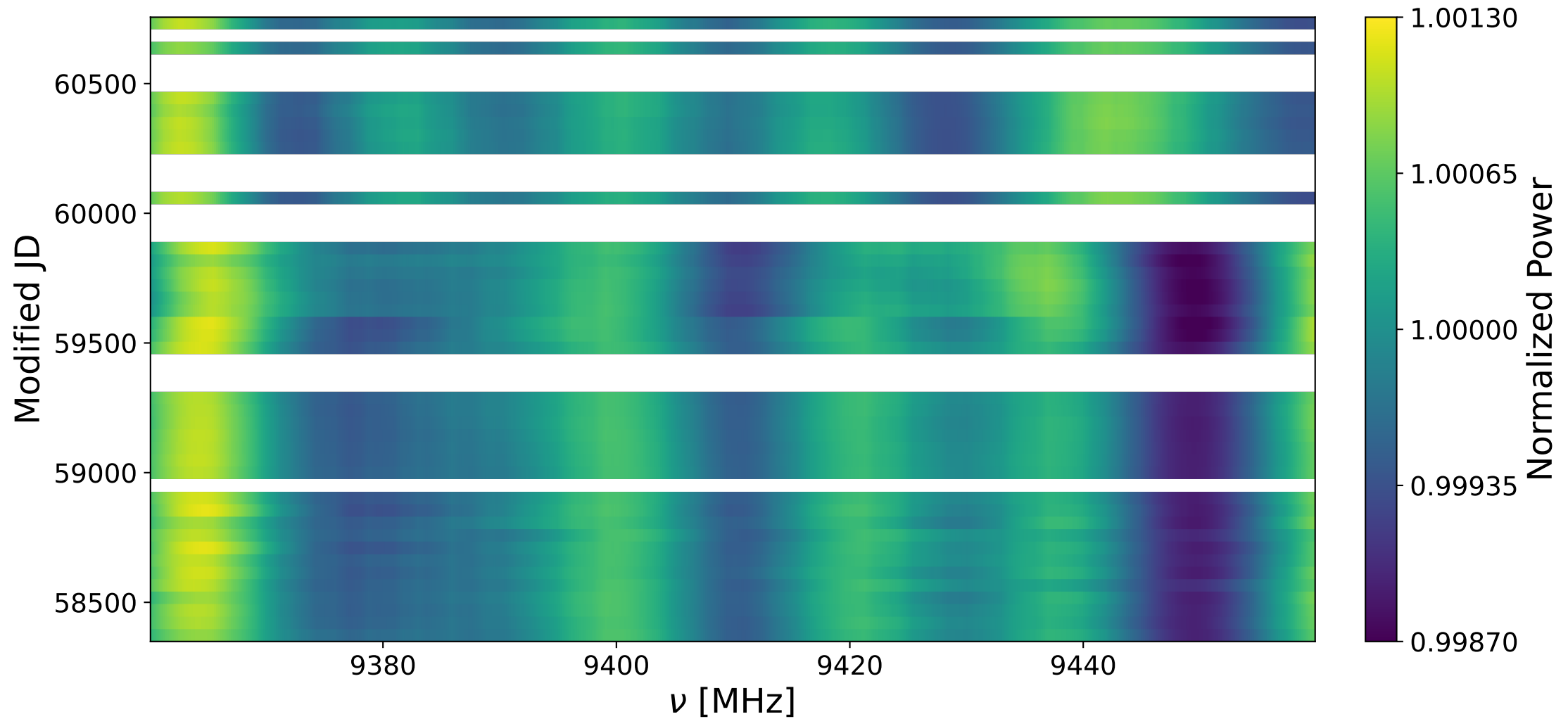
Bank 1 decay: 9360-9460 MHz
