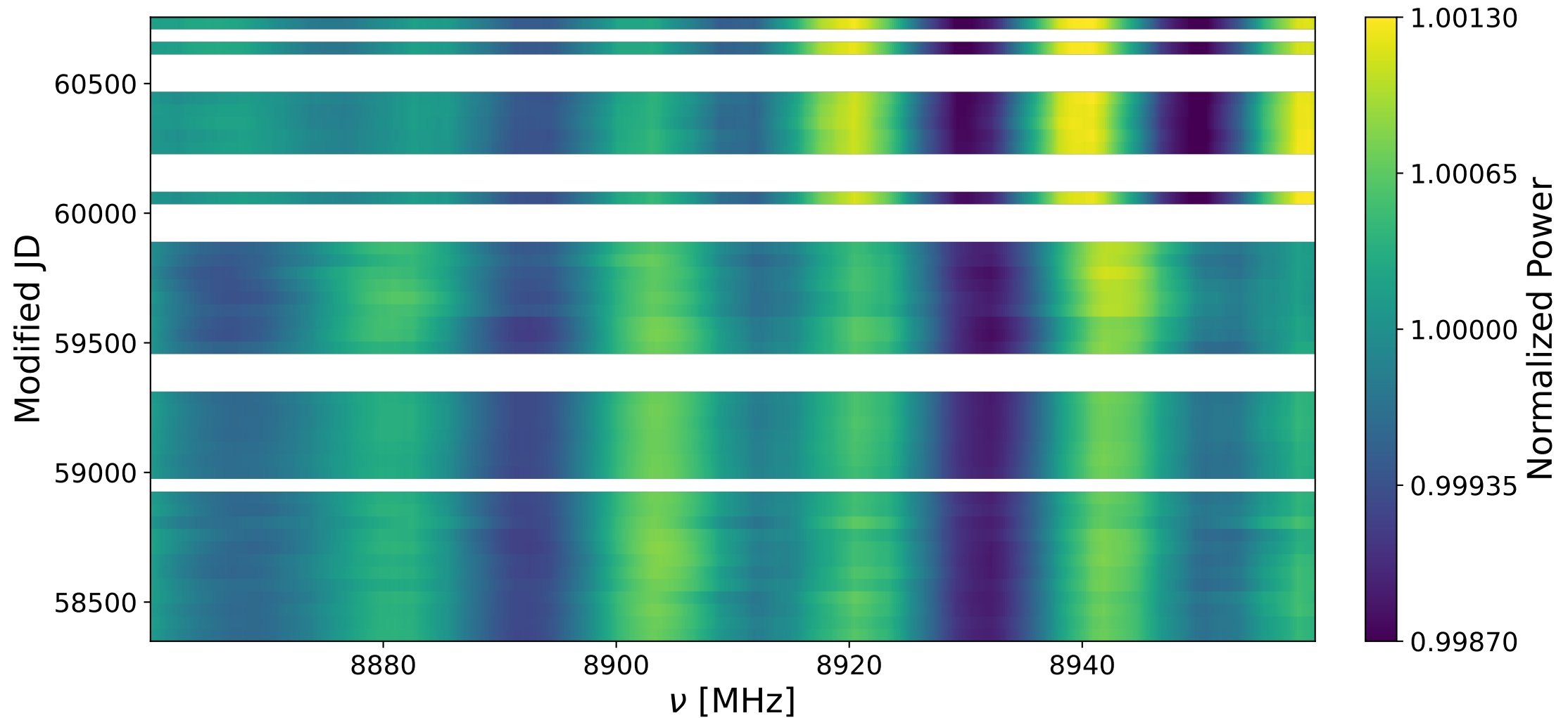
Bank 1 decay: 8860-8960 MHz
