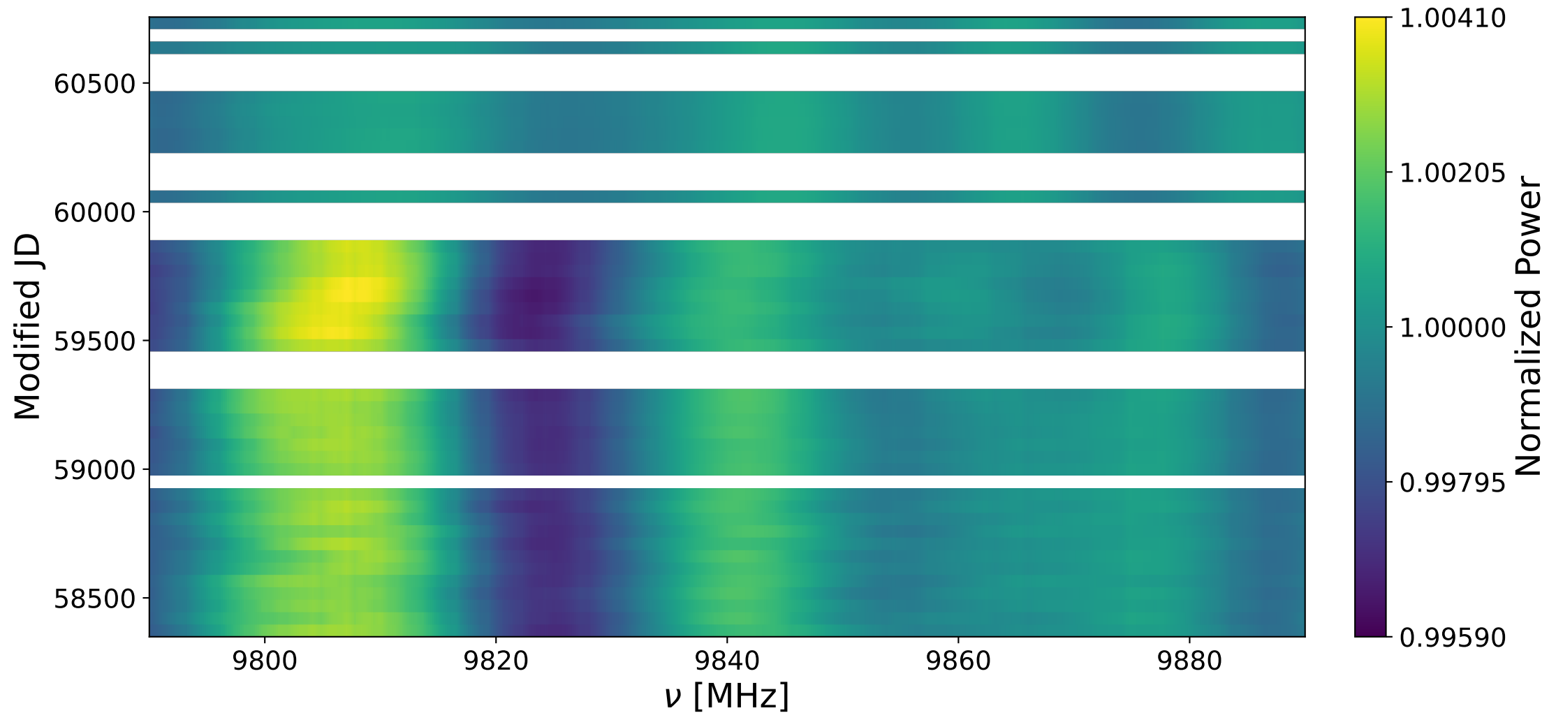
Bank 2 decay: 9790-9890 MHz
