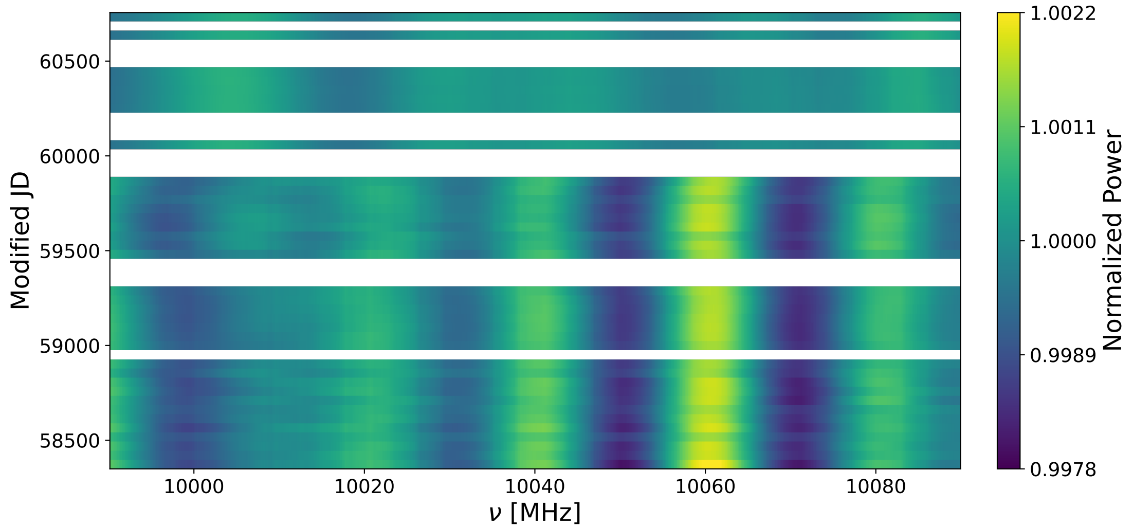
Bank 2 decay: 9990-10090 MHz
