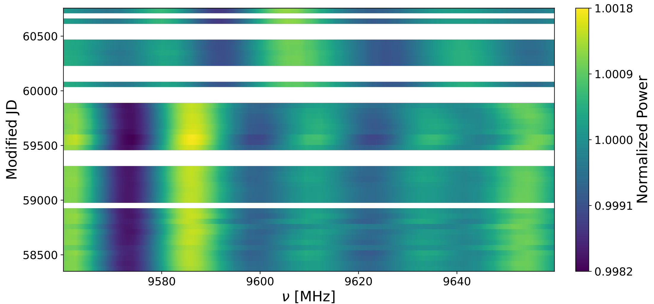
Bank 1 decay: 9560-9660 MHz
