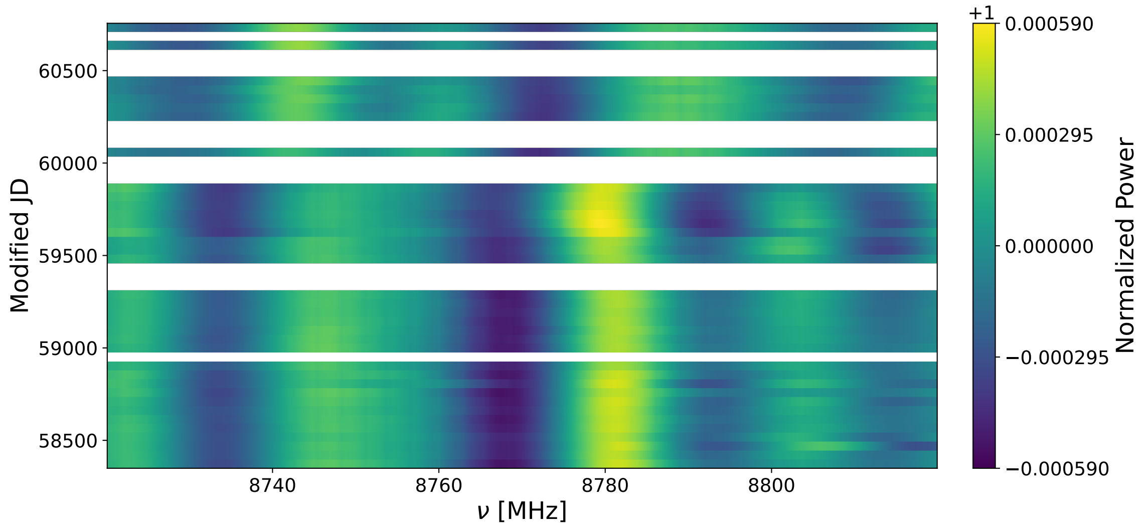
Bank 0 decay: 8720-8820 MHz
