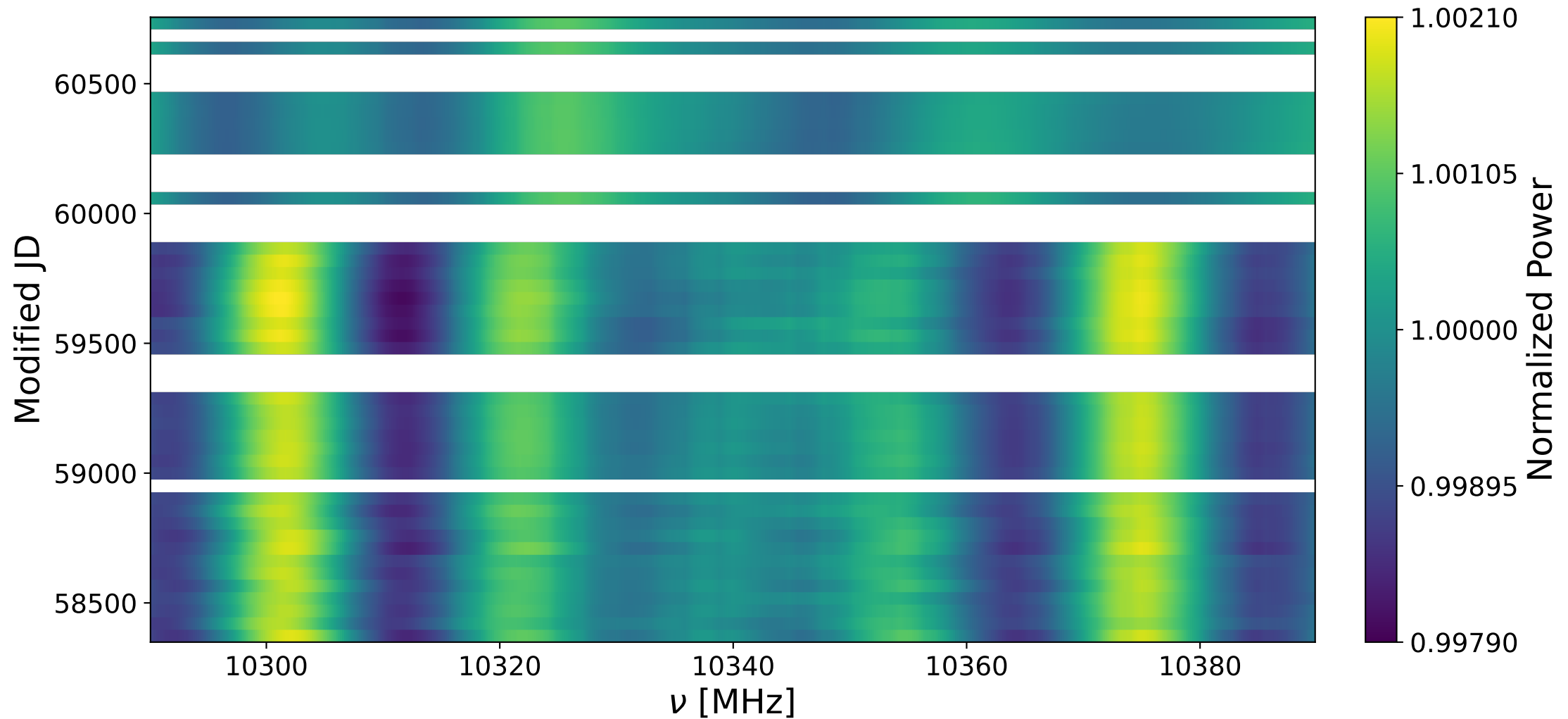
Bank 2 decay: 10290-10390 MHz
