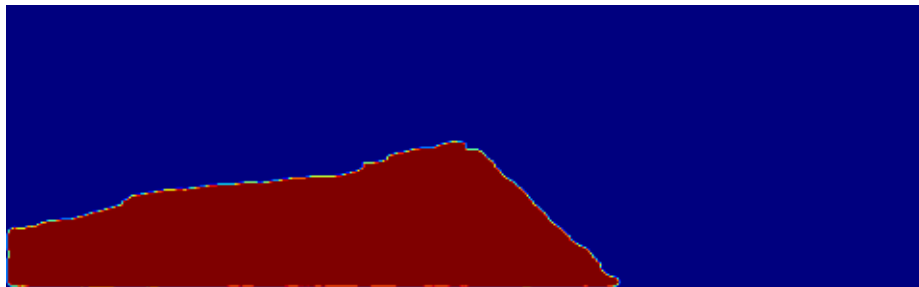
Predicted Mask
