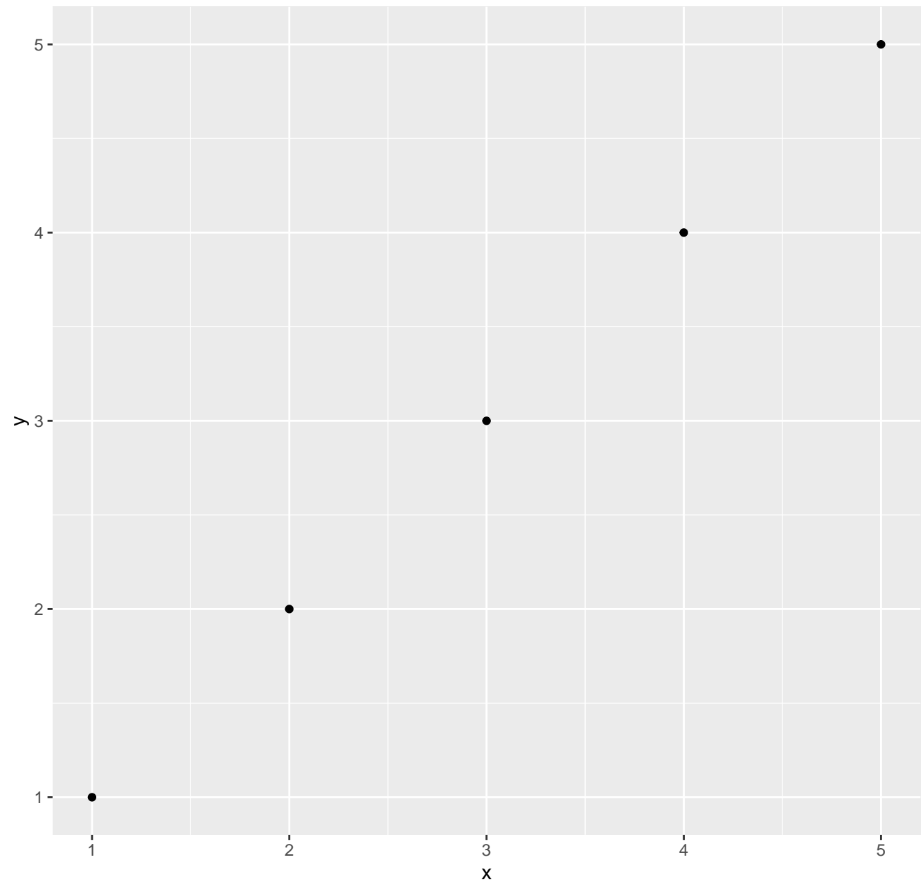
Normal Plot
