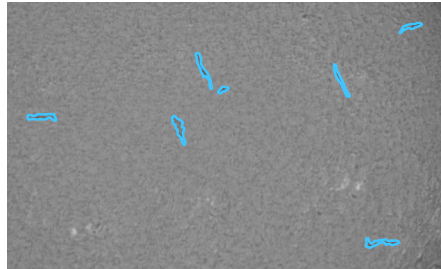
Final pipeline (7)
