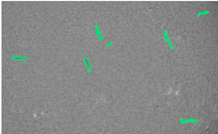
Annotation (7)
