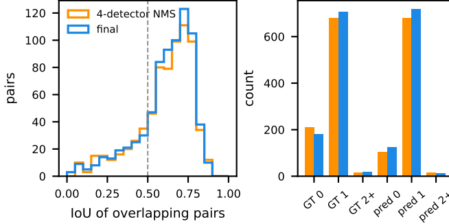
Fig. 5. The organizers’ overlap statistics on one calibration split. Left: IoU of every overlapping pair of prediction and annotation. Right: number of annotated filaments (GT) and predictions that overlap 0, 1, or 2 or more objects of the other kind. “GT 2+” corresponds to fragmentation (one-to-many) and “pred 2+” to merging (many-to-one).
