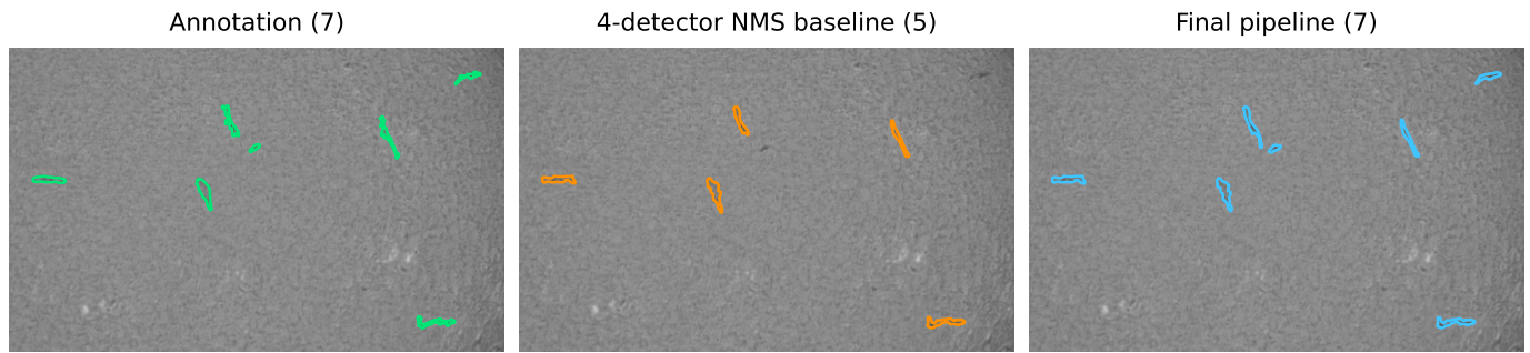
Fig. 6. A validation image on which the full system agrees well with the annotation (chosen among images with at least six annotated filaments as the one with the highest PQ for the full system, so it is a favorable case; the median image scores lower). Left: the outlines of one annotator. Middle: the four detectors find five of the seven filaments and miss the small one near the center and the one at the upper right. Right: the full system finds all seven.
