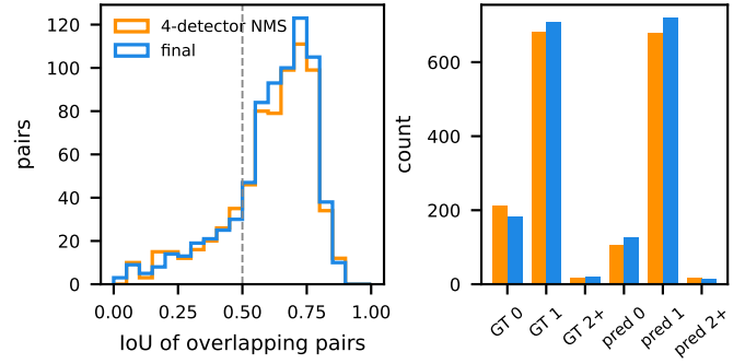
Fig. 4. Organizers’ overlap statistics on validation (one out-of-fold split). Left: \text{IoU} of every overlapping prediction–annotation pair. Right: number of annotated filaments (GT) and predictions overlapped by 0, 1, or \geq 2 partners; “GT 2+” is fragmentation (one-to-many), “pred 2+” merging (many-to-one).
