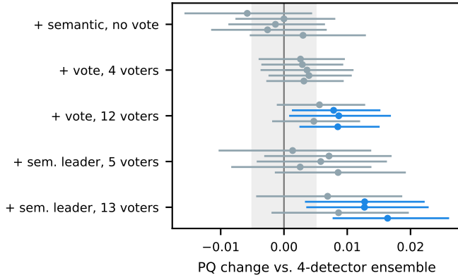
Fig. 3. PQ change versus the calibrated 4-detector ensemble on each of the five calibration splits (points) with paired-bootstrap 95% intervals; blue intervals exclude zero. The gray band marks \pm 0.005 , the change caused by retraining one detector with another seed.
