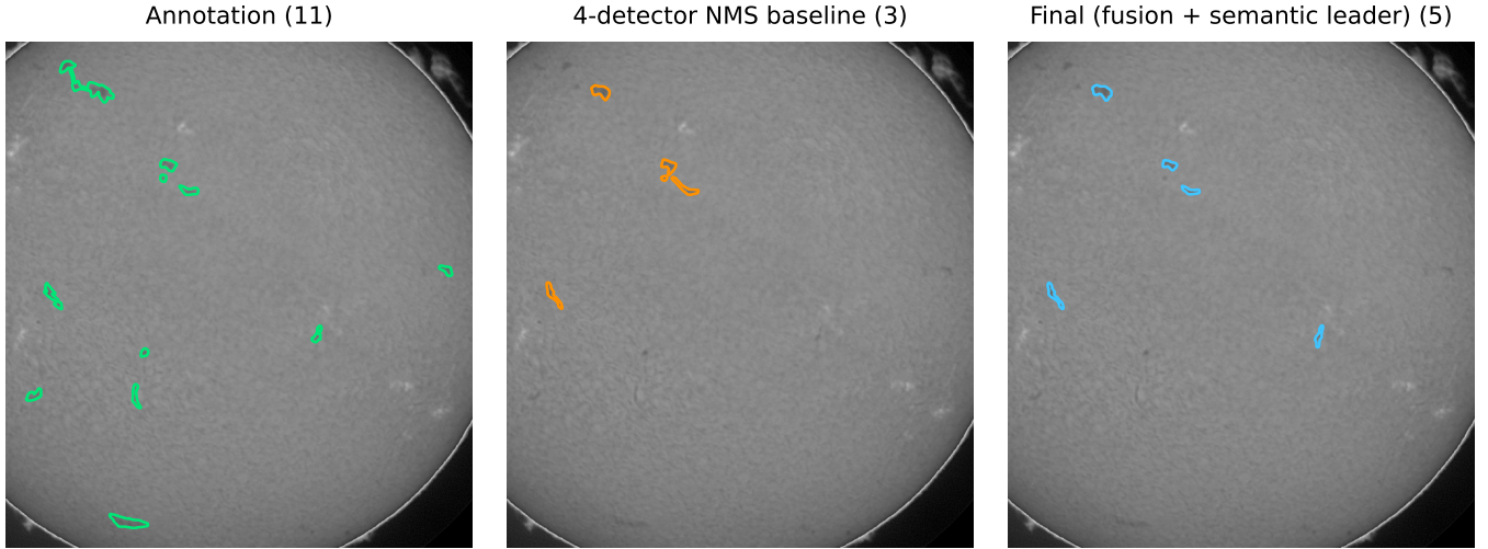
Fig. 5. Validation example where voting helps (chosen as the image with the largest gain in matched filaments, not as a typical case). Left: one annotator’s filaments. Middle: the 4-detector ensemble merges two filaments into one instance and misses several faint ones. Right: the final pipeline separates the pair and recovers two more; several faint annotated filaments remain undetected.
