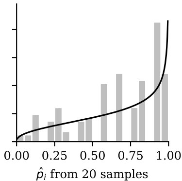
model B: Beta(1.41, 0.71)
