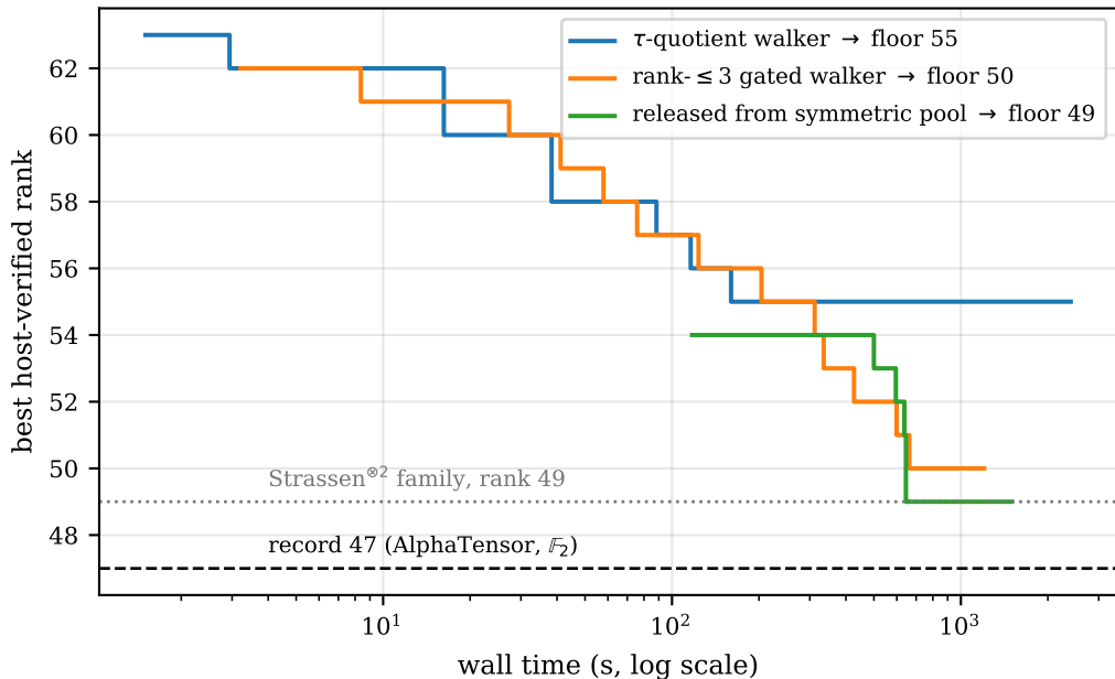
4 × 4 flip-walk dynamics: no walk crossed rank 49
