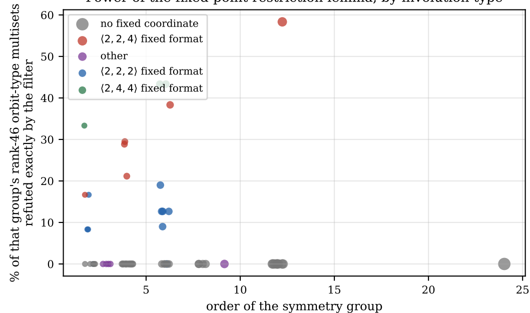
Power of the fixed-point restriction lemma, by involution type
