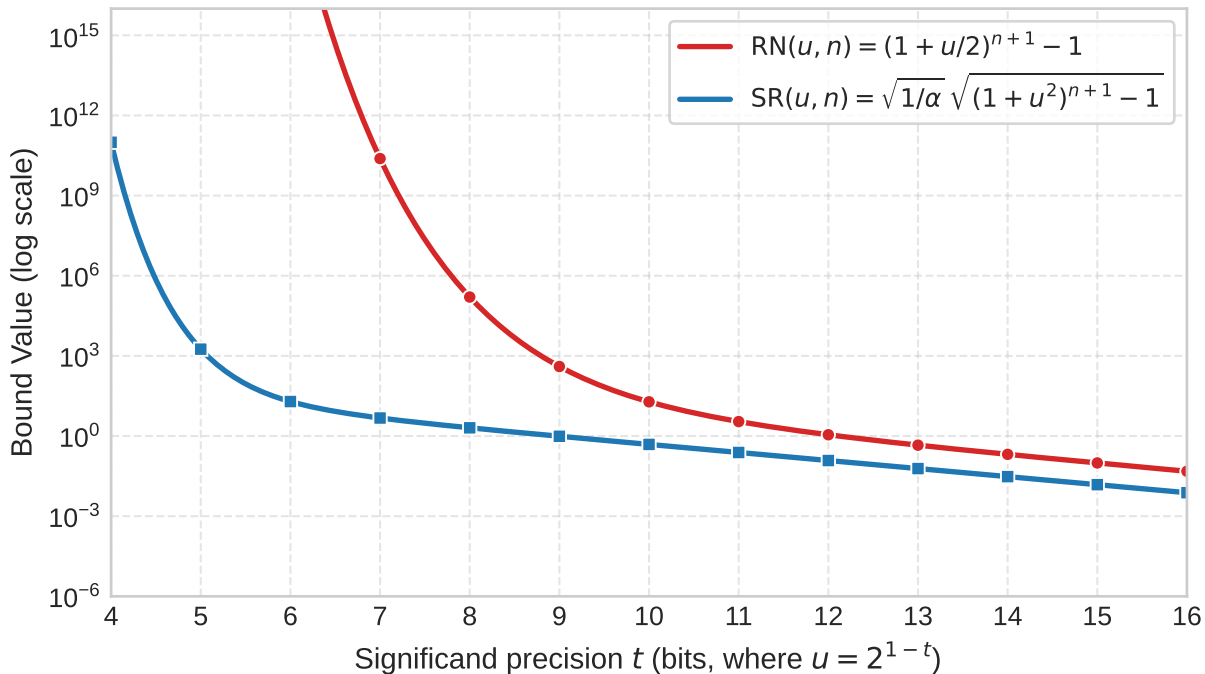
RN vs SR Error Bounds ( n = 3072, \alpha = 0.05 )
