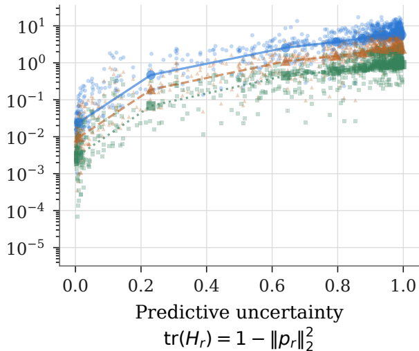
Language-model head
