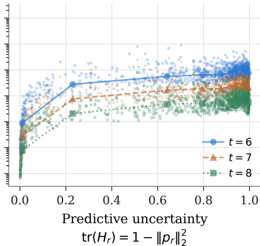
MLP down-projection
