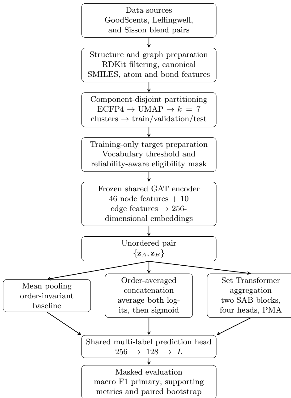
Figure 4.1: Compact overview of the proposed computational pipeline. The three aggregation branches receive the same frozen molecular embeddings and use the same prediction and evaluation protocol.
