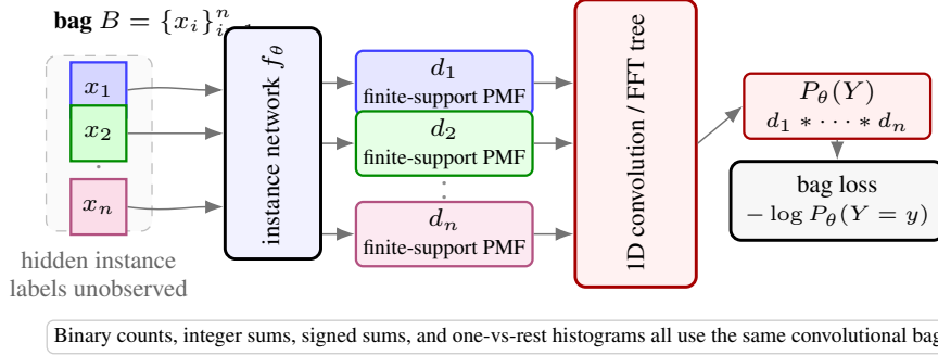
Figure 1: Convolutional aggregate pipeline. The instance network emits finite-support atomic PMFs d_i for each instance. A deterministic convolutional layer computes the aggregate PMF P_\theta(Y) , and the observed bag label selects the likelihood term used for training.
