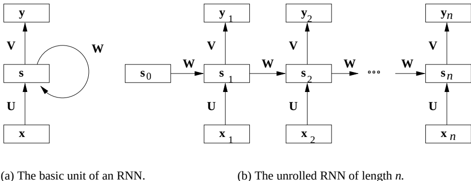
Figure 13.12: RNN architecture
