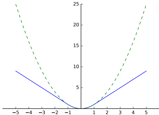
Figure 13.6: Huber Loss (solid line, \delta = 1 ) and Squared Error (dotted line) as functions of z = y - \hat{y}
