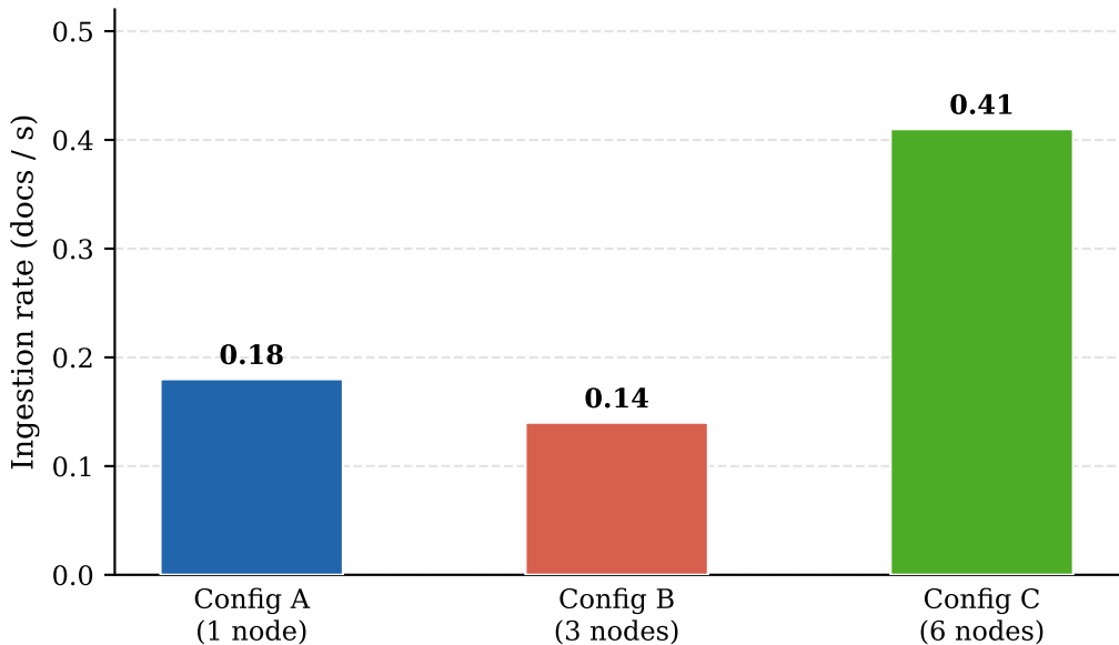
Phase 2 — Parallel ingestion throughput by cluster size
