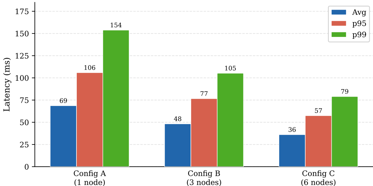
Phase 3 — Query latency percentiles by cluster size (50 concurrent, 30 s)
