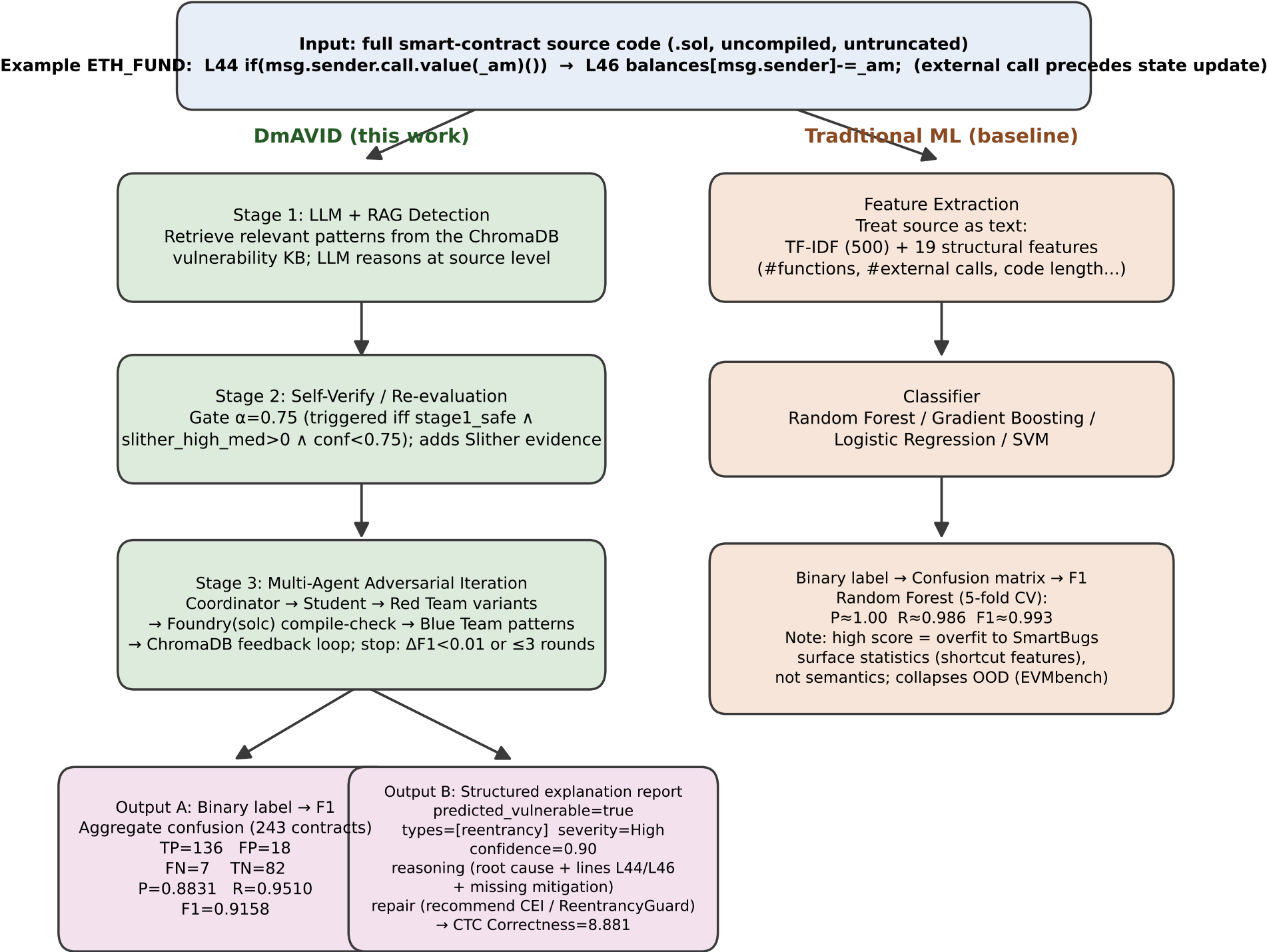
Figure A-1. DmAVID information-processing flow: from .sol source input to F1 score and vulnerability explanation report (traditional ML shown for contrast).
