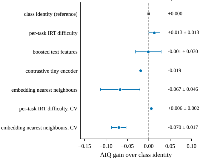
(a) instance features vs class identity
