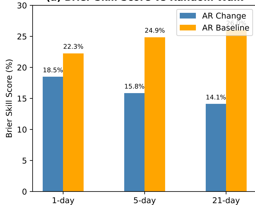
(a) Brier Skill Score vs Random Walk
