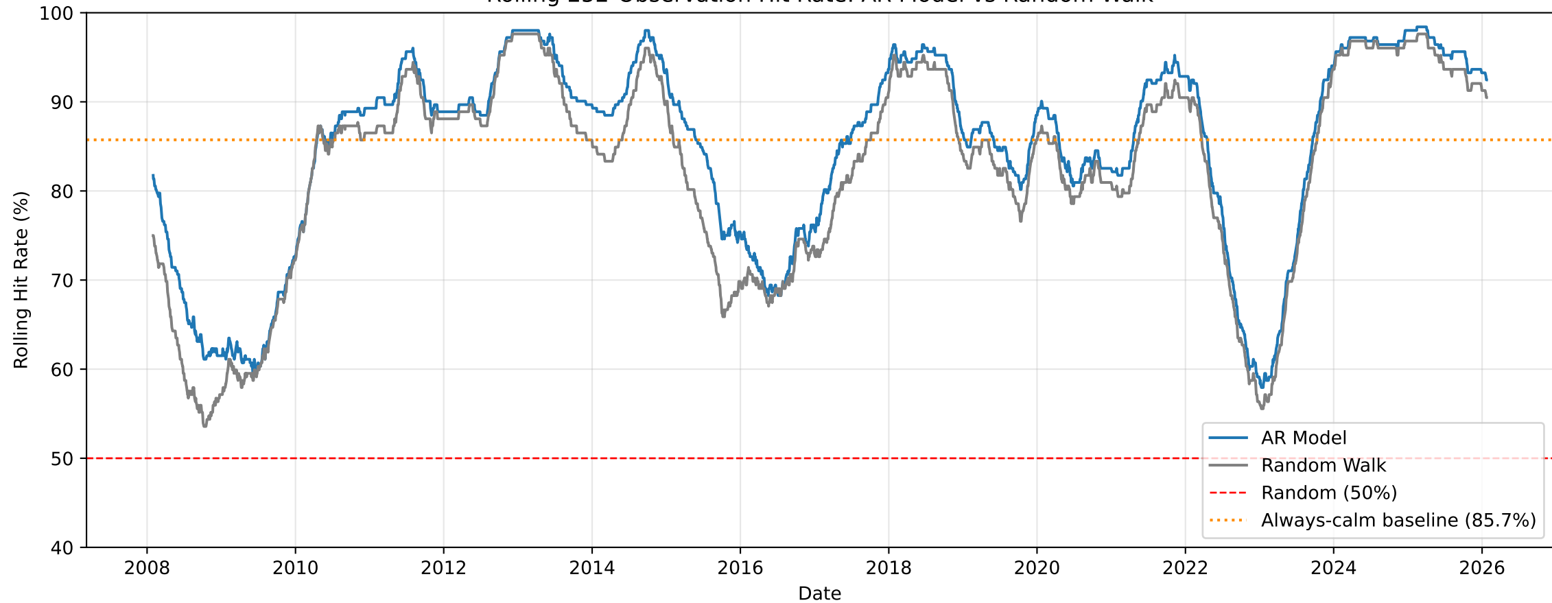
Rolling 252-Observation Hit Rate: AR Model vs Random Walk
