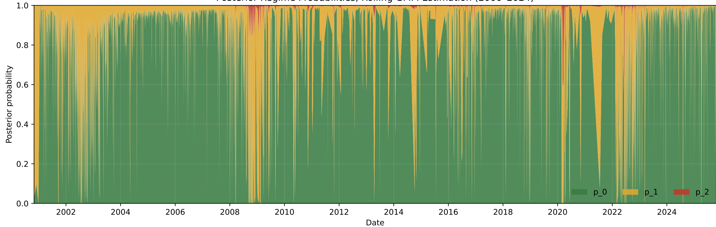
Posterior Regime Probabilities, Rolling GMM Estimation (2000-2024)
