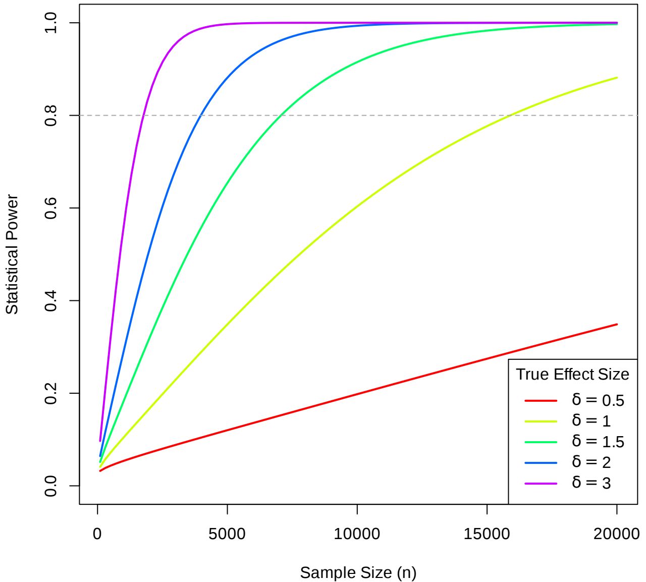
Power Curves with \sigma = 45 , H_0: \mu = 0
