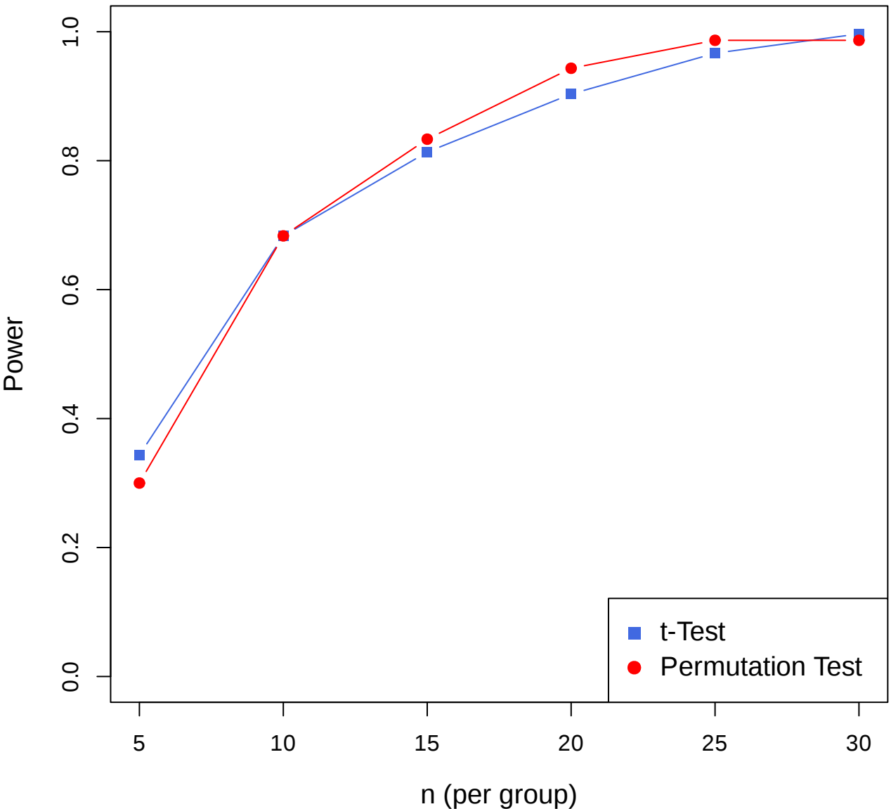
Power Curves: Normal Data, \delta=4.5 , \sigma=4
