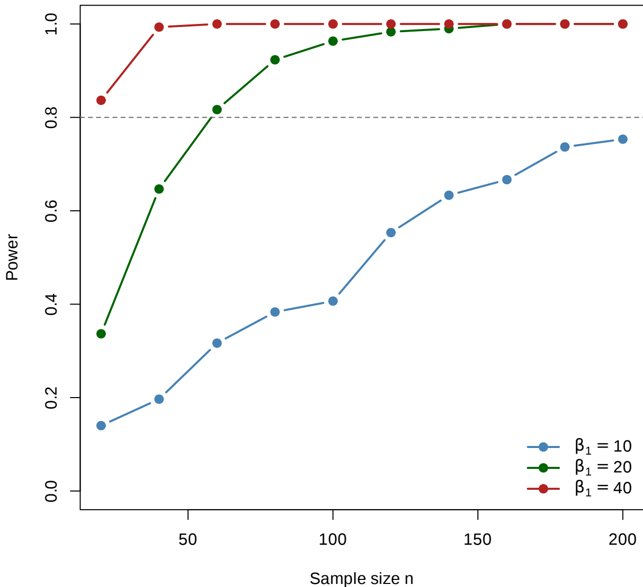
Power of the slope t-test vs. sample size (sigma = 150)
