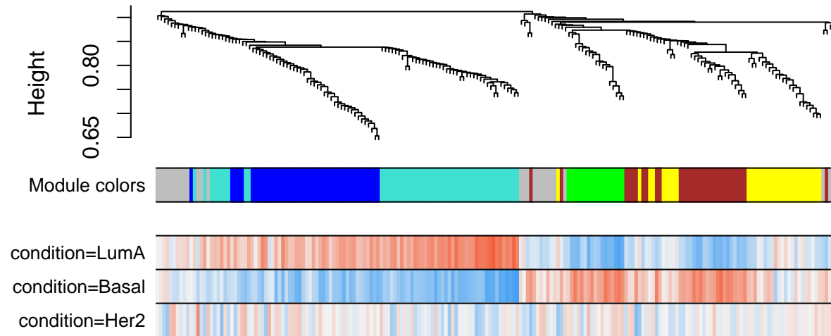
Dendro and colors GX
