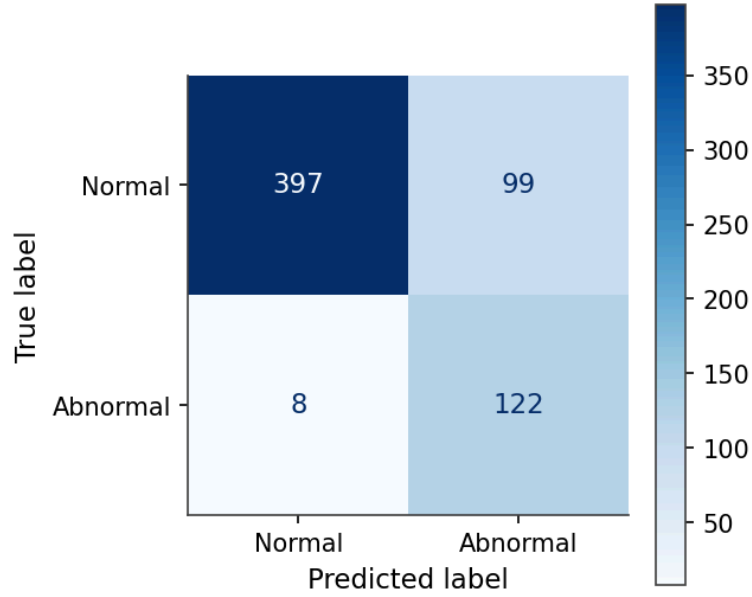
Figure 2 – Confusion matrix of the second-best heart-sound classical classifier (SVM, feature set B). Same test set as Figure 1.
