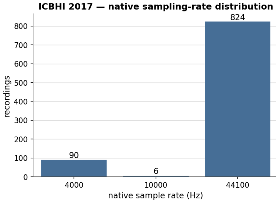
Figure 13 – Native sampling-rate distribution across ICBHI 2017 recordings. All recordings are resampled to 4 000 Hz before feature extraction.
