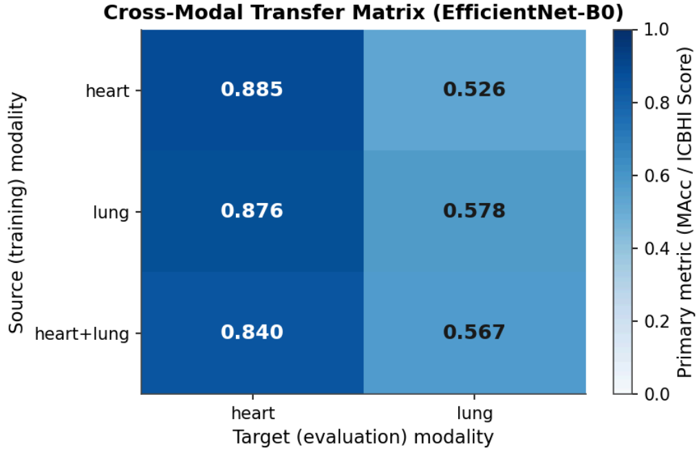
Figure 8 – Cross-modal transfer heat-map for the EfficientNet-B0 model. Each cell shows the primary metric (MAcc for heart; ICBHI Score for lung) when a model trained on the source modality (rows) is evaluated on the target modality (columns): the diagonal is in-domain, off-diagonal cells are direct transfer, and the bottom row is the joint multi-task model. The corresponding SmallCNN values appear in Table 3.
