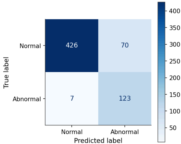
Figure 1 – Confusion matrix of the best heart-sound classical classifier (XGBoost, feature set B: MFCC+ \Delta + \Delta\Delta + spectral statistics). Rows: true class; columns: predicted class. Test set: 626 heart recordings (recording-level split; CinC 2016 publishes no recording-to-subject map — see Section 2.1).
