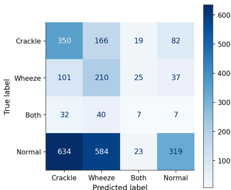
Figure 6 – Confusion matrix of the lung-sound SmallCNN classifier (on log-mel spectrograms). The log-mel representation enables better discrimination of crackle and wheeze relative to classical models.
