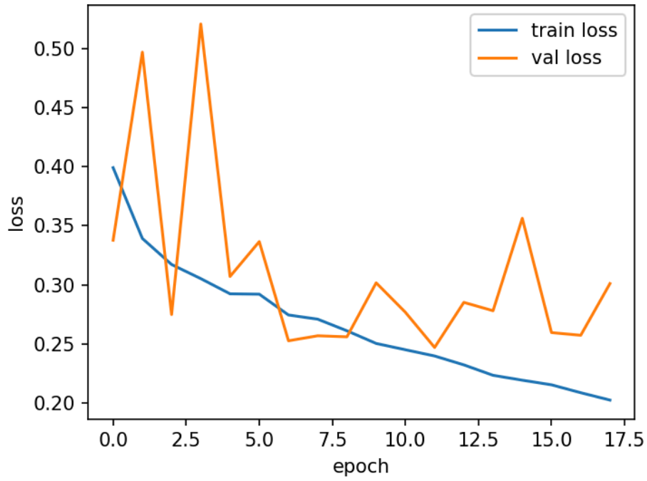
Figure 3 – Training and validation loss per epoch for SmallCNN on heart sounds. The training loss falls steadily and the (noisier) validation loss trends downward, indicating convergence without runaway overfitting.
