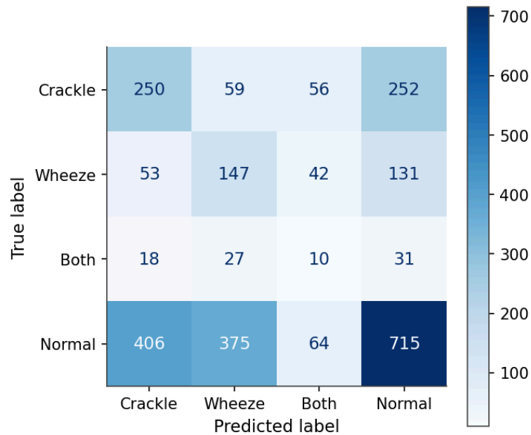
Figure 5 – Confusion matrix of the best lung-sound classical classifier (SVM, feature set B). Rows: true class; columns: predicted class. Test set: 2,636 cycles from 47 patients.
