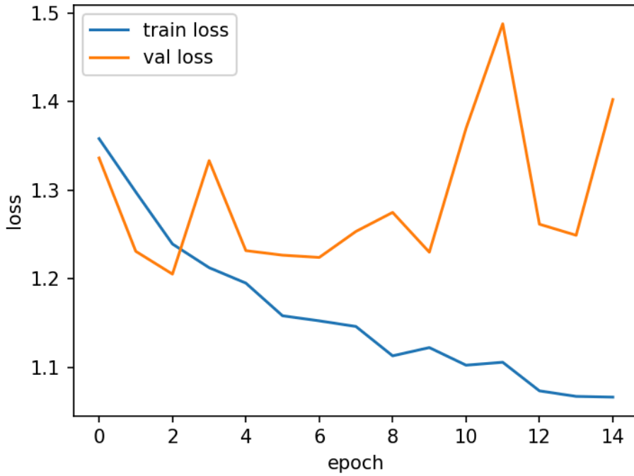
Figure 7 – Training and validation loss per epoch for SmallCNN on lung sounds. The validation loss starts rising after roughly epoch 9 (over-fitting on the harder four-class task), so early stopping restores the earlier best checkpoint.
