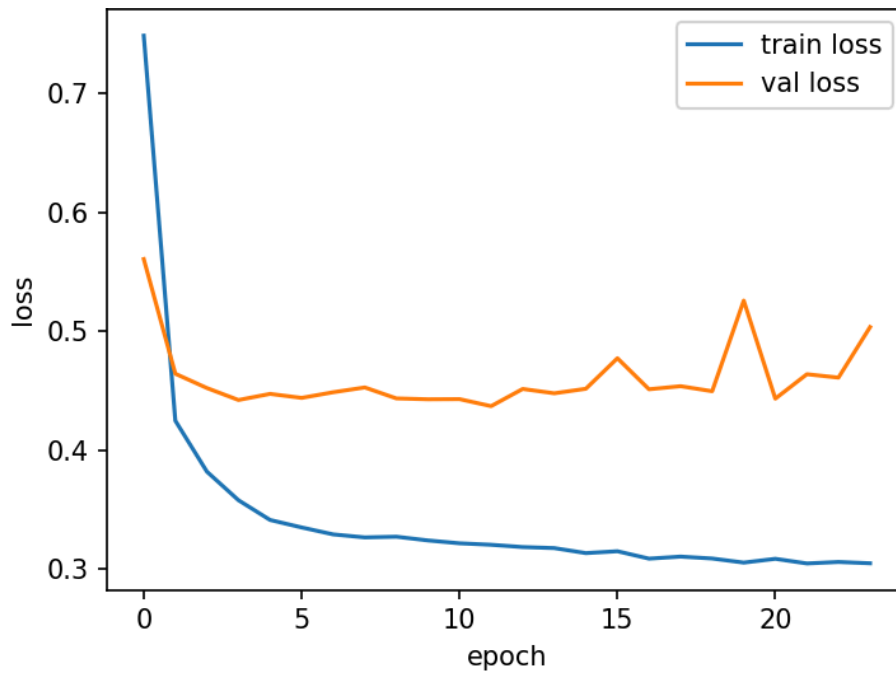
Figure 4 – Training and validation loss per epoch for EfficientNet-B0 on heart sounds. The validation loss plateaus while the training loss keeps falling — the modest train–validation gap typical of fine-tuning; early stopping selects the best checkpoint.
