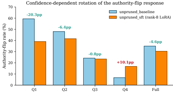
Figure 1. Confidence-dependent rotation of the authority-flip response. Clean SFT at rank 8 reduces flip rate at low baseline confidence (Q1 -20.3\text{pp} , Q2 -6.4\text{pp} ) and amplifies it at high baseline confidence (Q4 +10.1\text{pp} ). The full-pool average ( -4.6\text{pp} ) is dominated by Q1–Q2 in absolute count and hides both effects.
