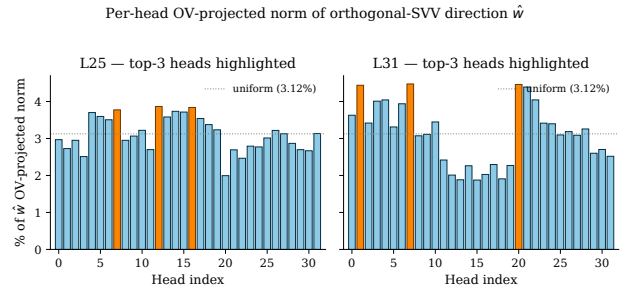
Figure 4. Per-head OV-projected norm fractions of the orthogonal-probe direction \hat{w} at L25 and L31. No head exceeds \sim 4.5\% ; top-10 cumulative is 36.85% / 40.88%; the distribution is close to uniform over the top \sim 20 heads per layer.
