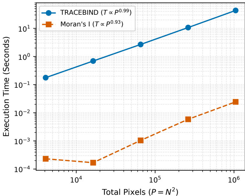
Runtime Scaling Complexity
