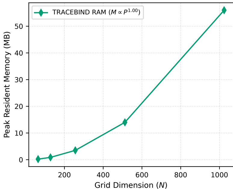
Memory Allocation Profile
