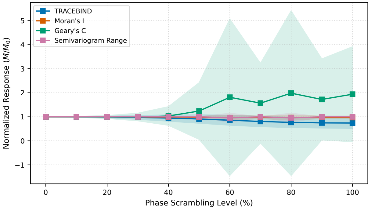
Benchmark 4: Diagnostic Decay Under Fourier Phase Randomization
