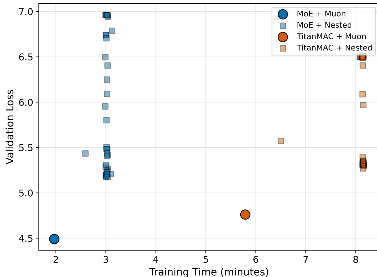
Time vs Performance
