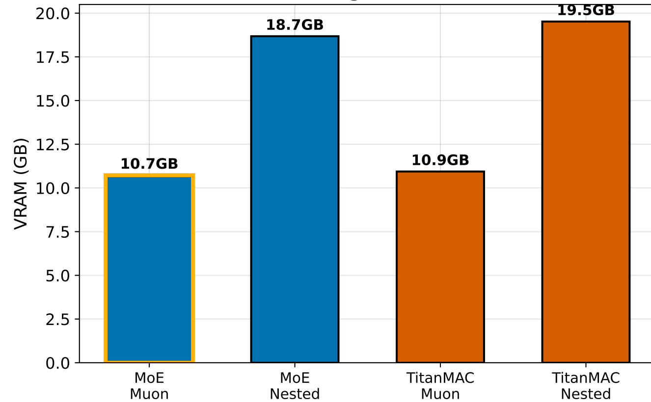
Peak VRAM Usage (lower is better)
