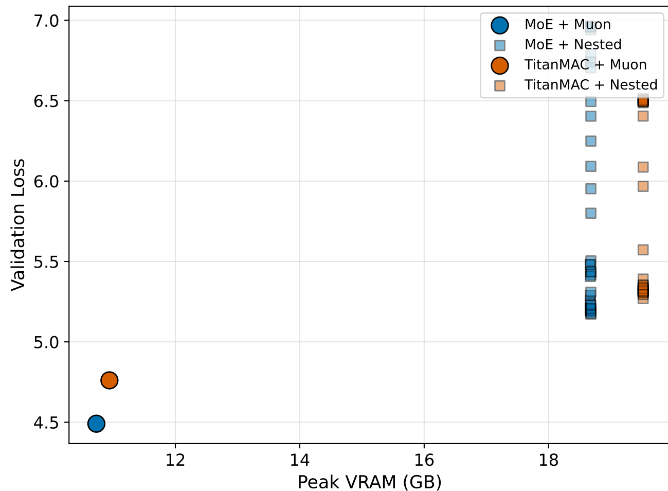
VRAM vs Performance
