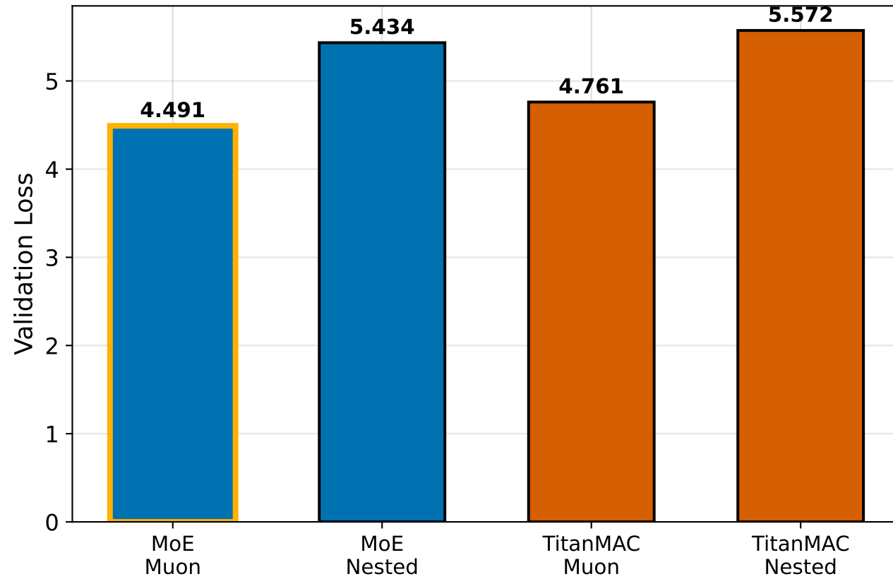
Validation Loss (lower is better)
