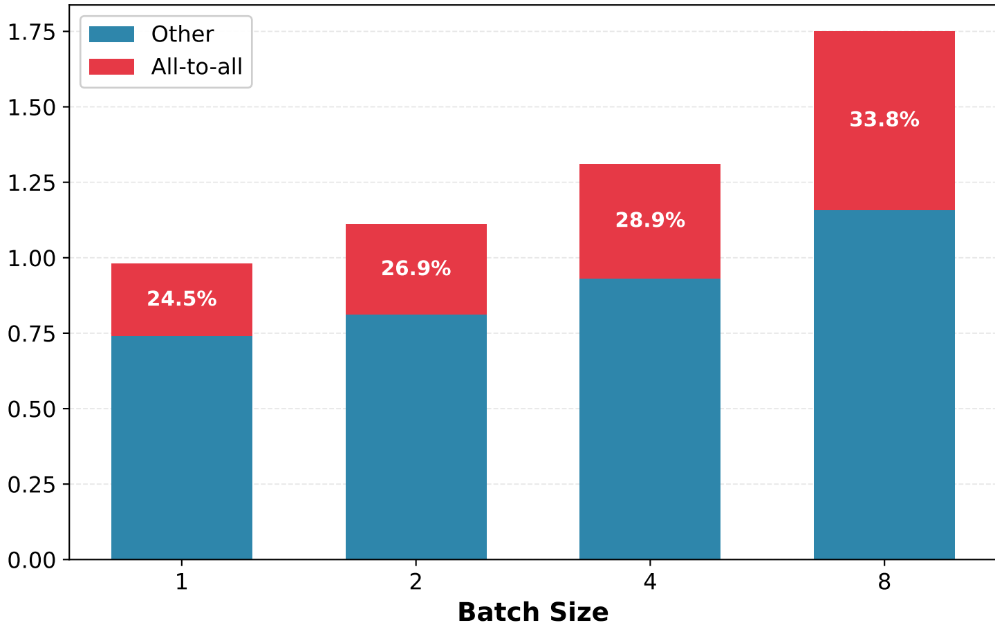
Average time per Iteration (s)
