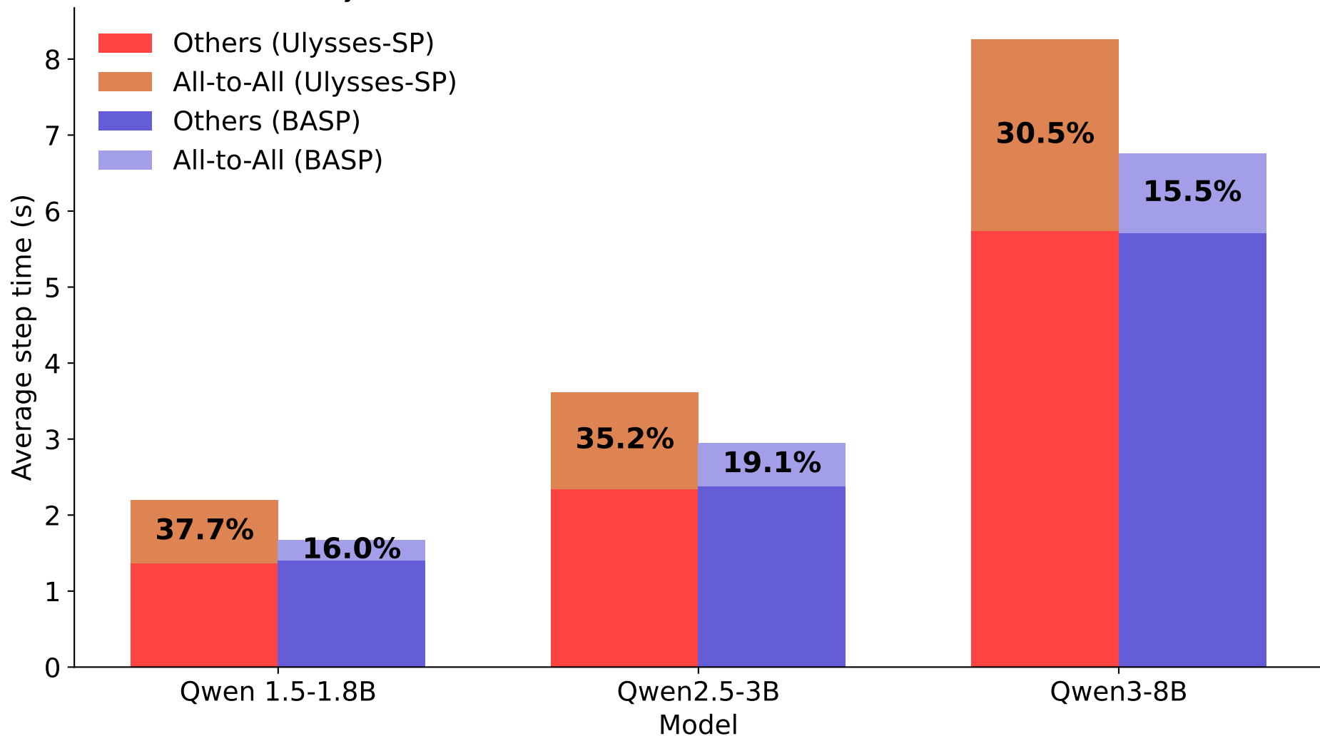
Ulysses-SP vs BASP with All-to-All Communication Portion
