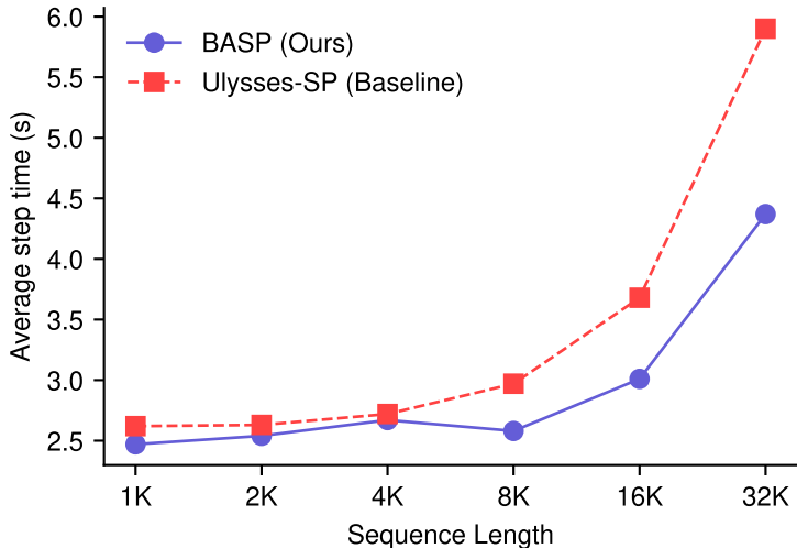
End-to-End Step Time (Batch Size=2)
