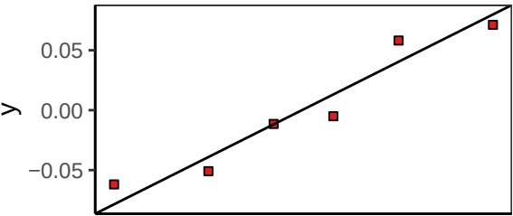
QQ Line Plot
