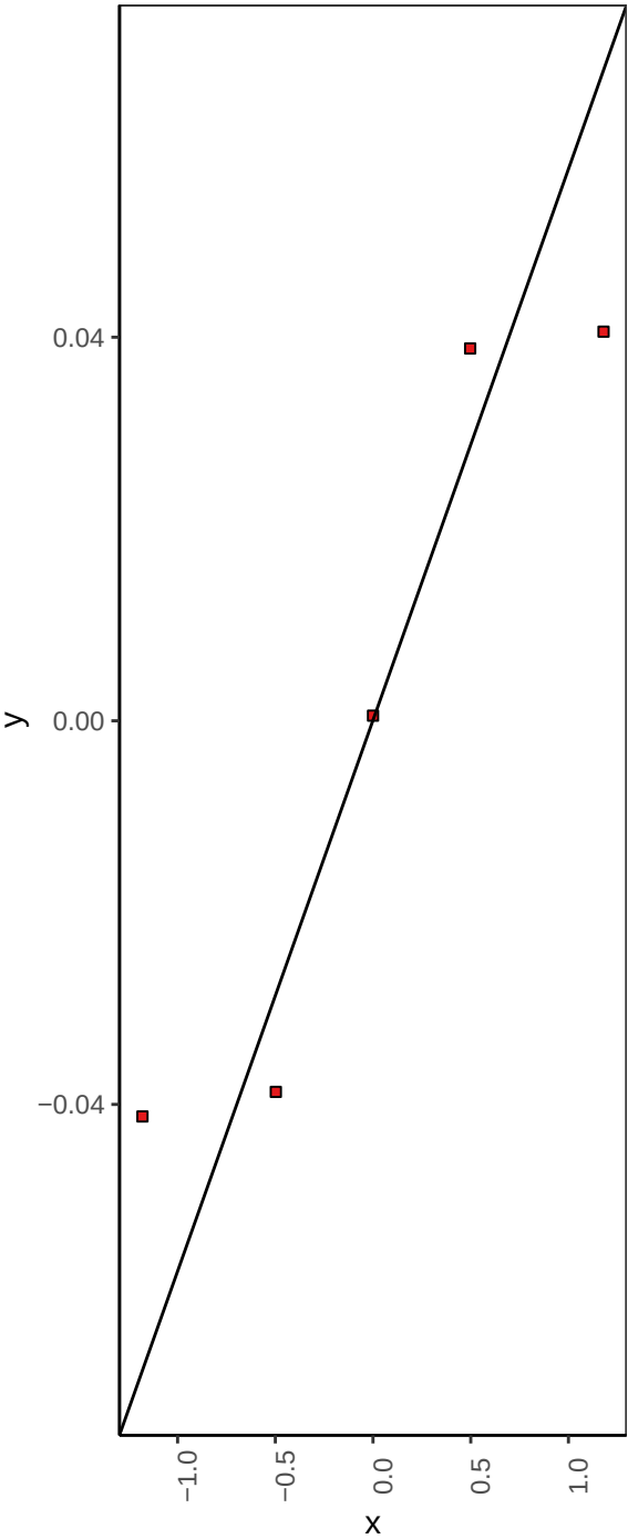
QQ Line Plot
