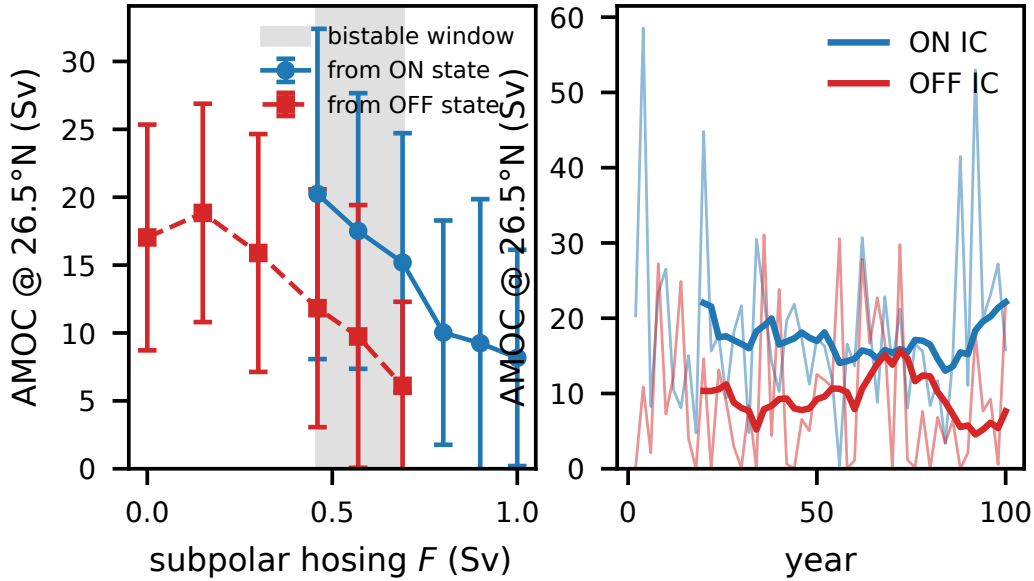
Figure 17.1: The AMOC hysteresis window. (a) On-state (blue) and off-state (red) equilibrated AMOC versus hosing F ; the branches stay separated across the window. (b) At F = 0.57 Sv the two initial conditions settle on different branches and do not reconverge over 100 years — the signature of genuine bistability.
