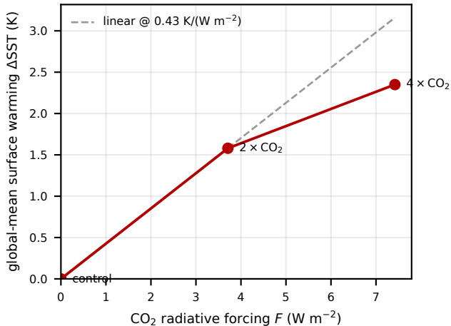
Transient forcing response (TCR-like proxy)
