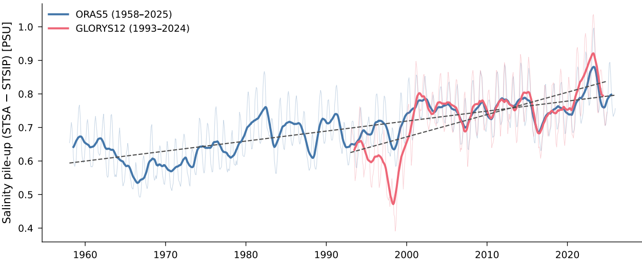
Salinity pile-up index: multi-product comparison
