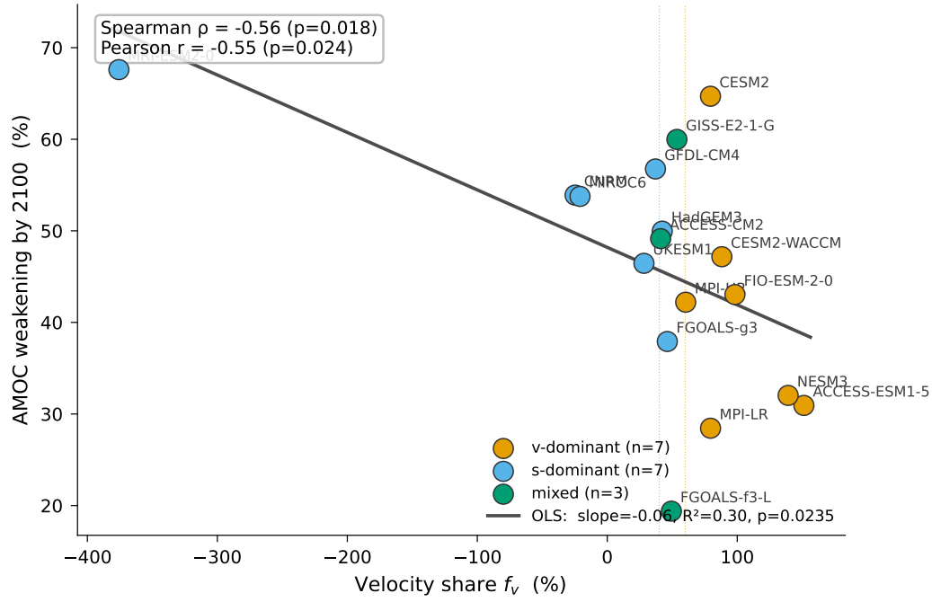
Figure S6: Continuous velocity-share vs projected AMOC weakening. Across the 17 forced-weakening CMIP6 models with AMOC26N output, the velocity-share f_v and the percent AMOC weakening by 2100 (2081-2100 vs 1950-1980) carry a Spearman rank correlation of \rho = -0.56 ( p = 0.018 , two-sided) and a Pearson r = -0.55 ( p = 0.024 ). The OLS regression has slope -0.063\% weakening per percent f_v and R^2 = 0.30 . The continuous correlation is significant at the 5% level and independently confirms the binary mechanism-class partition reported in Main Fig. 2(c) (salinity-dominant models project more weakening). The expansion from n = 12 in v4.3 to n = 17 here was achieved by dedicated extraction of msftmz (or msfityz ) for the v4.3-added models that publish a meridional streamfunction.
