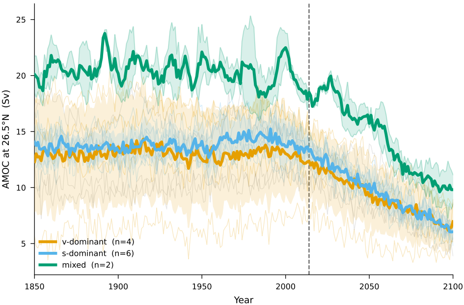
(a) AMOC trajectories by F_{ovS} mechanism class
