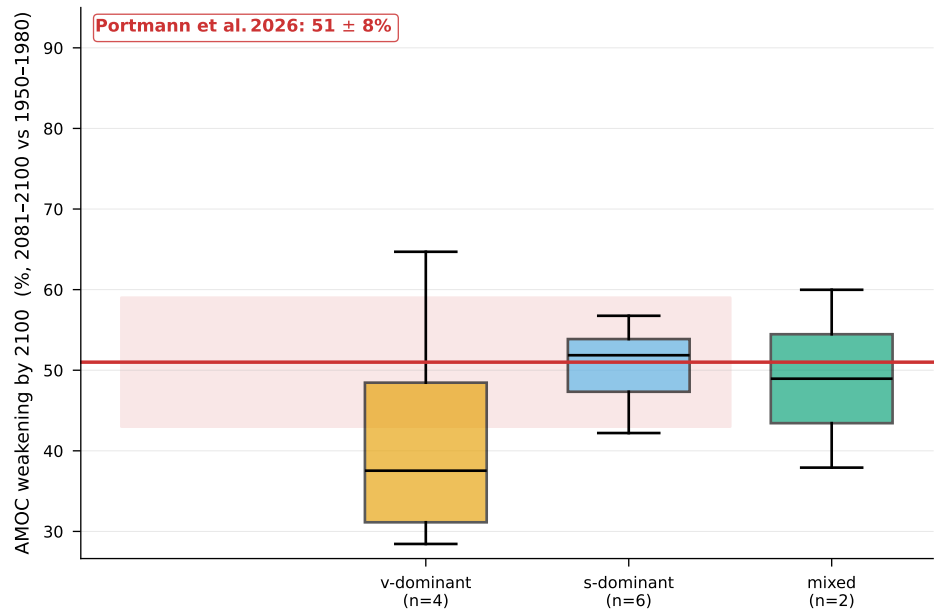
(b) Projected weakening conditional on mechanism
