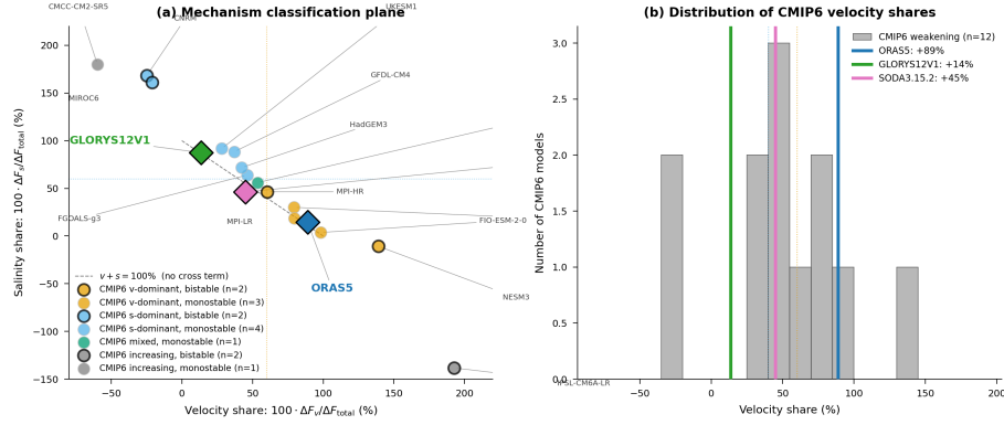
Figure 3: CMIP6 tie-breaker: observational reanalyses span the full mechanistic spectrum of coupled-model responses. (a) Velocity-share vs. salinity-share for the 12 forced-weakening CMIP6 models; symbol edge colour encodes baseline regime (black = bistable F_{\text{ovs}} < 0 , grey = monostable), and symbol face colour encodes mechanism class. ORAS5 (blue diamond), GLORYS12V1 (green), SODA 3.15.2 (pink), and ECCO-V4r4 (red) are overlaid. The reanalyses bracket the full CMIP6 physical diversity along the velocity/salinity axis. (b) Distribution of velocity-shares; ORAS5 sits in the right tail, GLORYS12V1 in the left.
