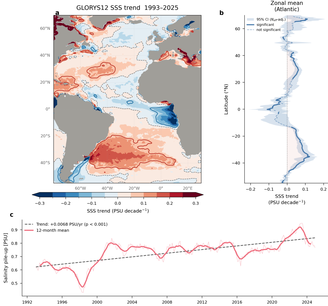
Figure 4. GLORYS12V1 SSS trends and salinity pile-up (1993–2025). (a) Per-pixel deseasonalized linear SSS trend (PSU decade -1 ) with significance stippling (hatching where p \geq 0.05 ). (b) Atlantic zonal-mean SSS trend profile with 95% confidence intervals adjusted for spatial autocorrelation ( N_{\text{eff}} ; Bretherton et al. (1999)). Solid segments indicate statistically significant trends; dashed segments are not significant. (c) Salinity pile-up index time series with linear trend (+0.007 PSU yr -1 , p < 0.001 ).
