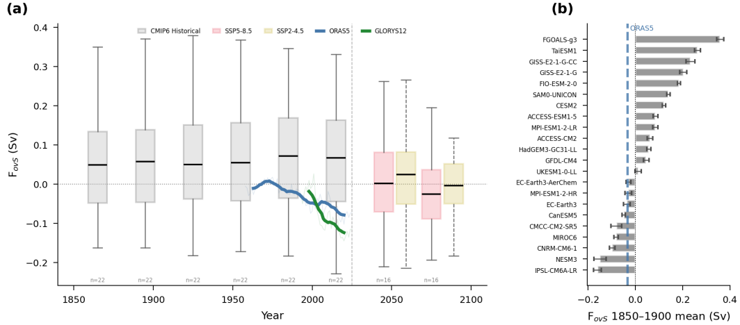
Figure 6. Observed vs. modeled F_{ovS} . (a) 30-year epoch box plots of CMIP6 model F_{ovS} means (historical: grey; SSP5-8.5: red; SSP2-4.5: yellow). Overlaid: ORAS5 (blue) and GLORYS12V1 (green) as continuous time series (faint: annual means; bold: 10-year running means). The dashed vertical line marks the present (2025). (b) Historical-experiment mean F_{ovS} for 22 CMIP6 models, sorted by value. Models with negative means reside in the bistable regime. The observed ORAS5 mean ( -0.033 Sv, blue dashed line) falls among the bistable models, while roughly half the CMIP6 ensemble maintains F_{ovS} > 0 (monostable).
