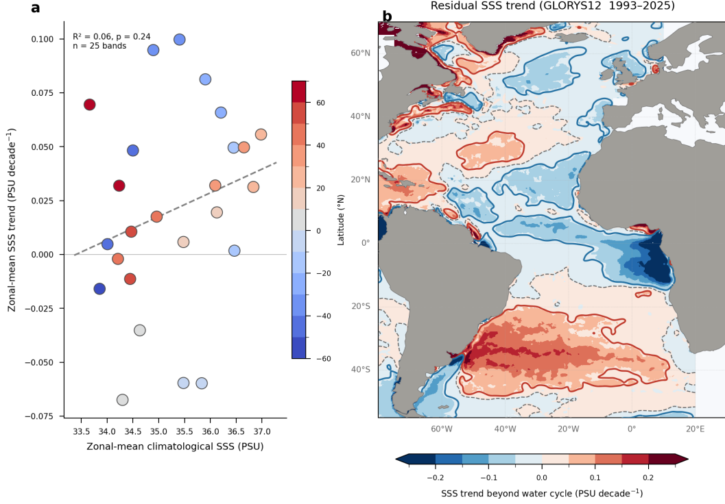
Figure 5. Decomposition of Atlantic SSS trends into hydrological cycle and ocean dynamics components (GLORYS12V1, 1993–2025). Zonal-mean climatological SSS versus zonal-mean SSS trend across 25 latitude bands, colored by latitude. The dashed line shows the amplification regression ( R^2 = 0.06 , p = 0.24 ), which predicts that SSS trends should mirror the mean pattern under greenhouse-driven water cycle intensification. The weak relationship indicates that ocean dynamics, not the hydrological cycle, dominate Atlantic SSS trends.
