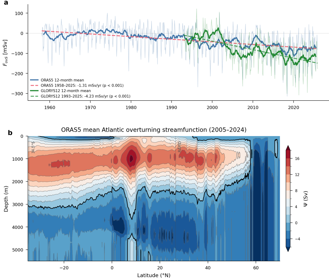
Figure 1. (a) Overturning freshwater transport at 34.5^{\circ}\text{S} ( F_{ovS} ) from ORAS5 (1958–2025, blue) and GLORYS12V1 (1993–2025, green). Monthly values (faint) with 12-month running means (bold). Dashed lines show linear trends for each product and period. The horizontal dotted line marks F_{ovS} = 0 ; negative values indicate the bistable regime where the salt-advection feedback is self-amplifying. (b) Time-mean Atlantic meridional overturning streamfunction \Psi(\phi, z) from ORAS5 (2005–2024, 240 months). Contours show the clockwise upper cell (positive, Sv) and the deep counter-clockwise cell (negative). The maximum of the upper cell defines the AMOC strength.
