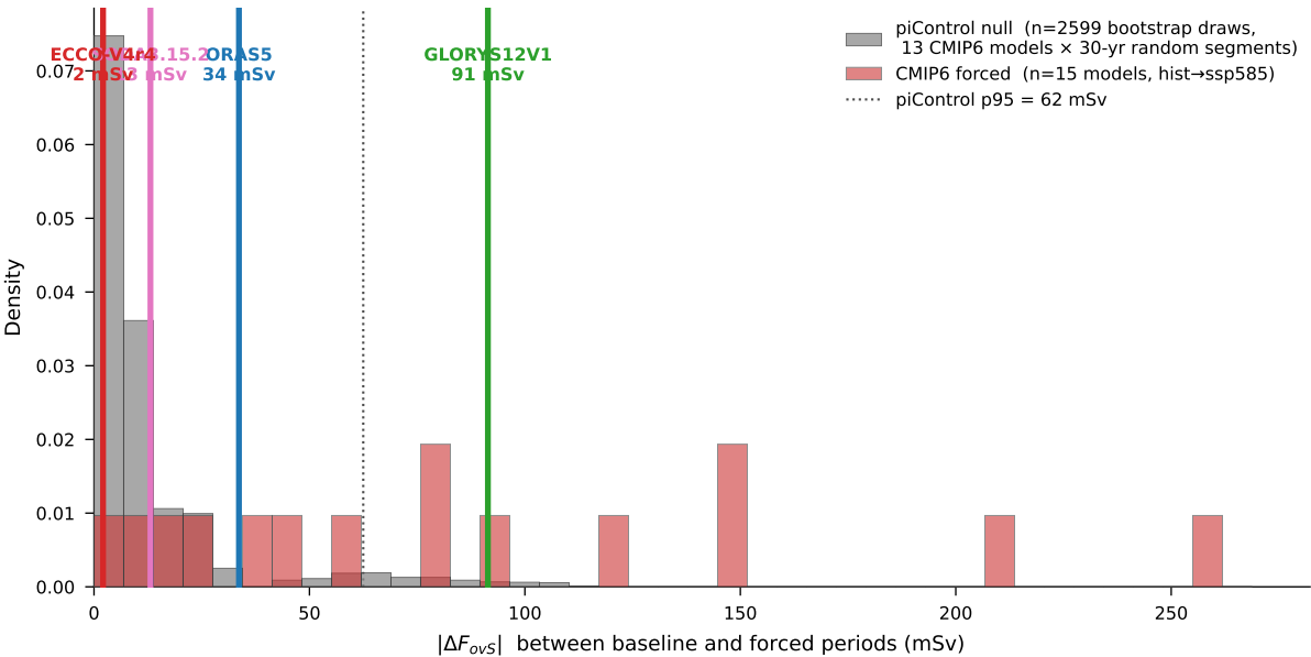
Fig. S4 — Signal-to-noise: forced \Delta F_{ovS} vs internal-variability null
