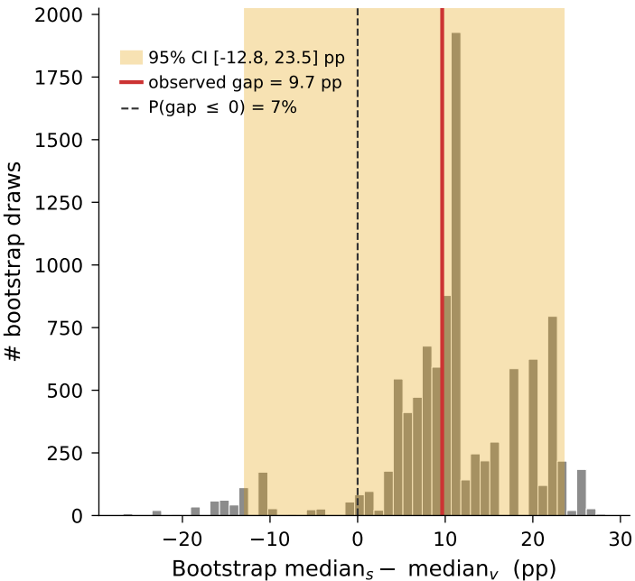
(a) standard ( n_v = 5 , n_s = 6 )
