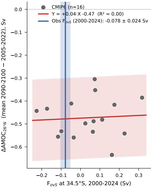
(a) CMIP6 emergent constraint
