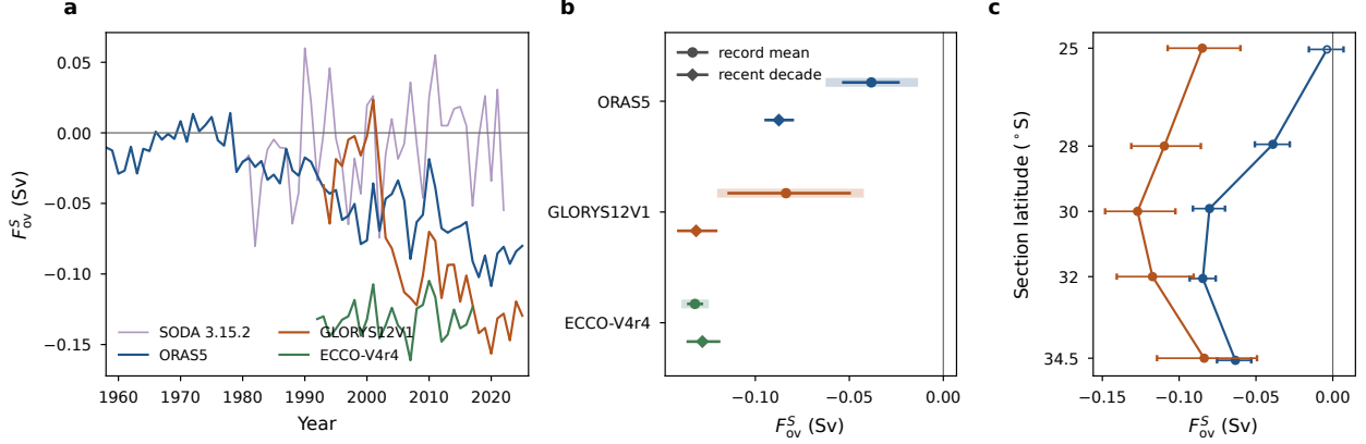
Figure 1. Overturning freshwater transport at 34.5°S in four ocean reanalyses. The sign of the overturning freshwater transport at 34.5°S. a , Annual-mean F_{ov}^S for ORAS5 (1958–2025), GLORYS12V1 (1993–2025), ECCO-V4r4 (1992–2017) and ECCO-V4r4 are computed here from monthly fields on the contiguous Atlantic section; SODA 3.15.2 (1980–2022); horizontal lines mark each record means carried over from an annual-field pipeline, is not on the same basis, and is not used in any quantitative claim. b , Record means mean (circles) and most recent decade (diamonds) with 95% circular block-bootstrap confidence intervals, at a 5-year blocks block for the record mean and a 3-year block for the decade. The pale bar spans the intervals obtained for block lengths of 2 to 20 years. Between-product spread is 0.094 Sv, 10 wider than the widest of these intervals (0.073 Sv, 000 iterations GLORYS12V1 across block lengths) ; solid and 1.5 times the 5-year intervals exclude zero, dashed do not quoted in the text. c , Mean F_{ov}^S trends over each product's own record (circles) and over 1993–2025 against section latitude, with the common 1993–2017 window (diamonds). Filled markers indicate a Santer-adjusted p < 0.05 same intervals. No product has a significant trend in The open marker is the common window one case whose interval includes zero.
