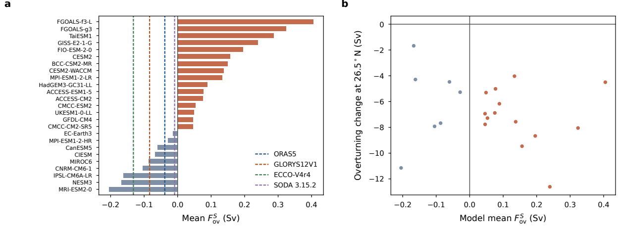
Figure 4. CMIP6 sits on the other side of zero, and the sign does not predict the rate. CMIP6 lies above the observational estimates, but cannot be sorted by the sign of F_{ov}^S . a, Historical mean Mean F_{ov}^S at 34.5°S over 1950–1980 in 25 CMIP6 models, with the four reanalysis estimates marked; 16 of 25 SODA is shown for continuity with Fig. 1 and is not used quantitatively. No offset or bias correction is applied to either models or reanalyses. b, Model mean F_{ov}^S against the 2005–2023 overturning trend change at 26.5°N for from 1850–1900 to 2081–2100 in the 16–21 models with the required output, with the RAPID, ORAS5 and GLORYS12V1 estimates for the same window. The two quantities are uncorrelated historical plus ssp585 projections (Pearson r = -0.04 , r = -0.20 , p = 0.88 ; Spearman \rho = +0.07 , p = 0.40 , p = 0.79 smallest reachable |r| = 0.43 ). Model numbering—This replaces a 19-year single-member trend test, whose null result is given in Extended Data Table—guaranteed by internal variability: 19-year trends span -3.5 to +2.4 Sv per decade across 50 members of the MPI-ESM1-2-LR large ensemble.
