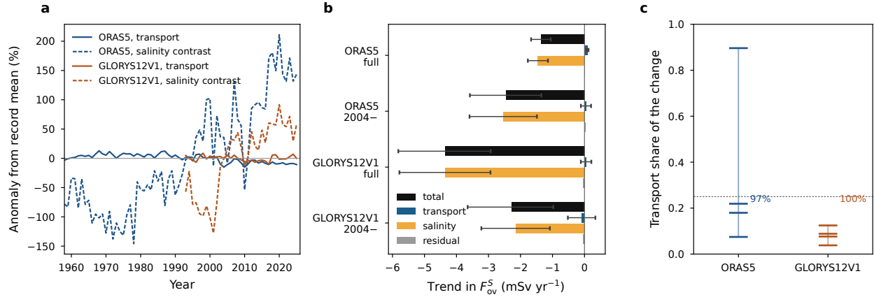
Figure 2. The decline in F_{ov}^S is not a change in overturning strength. The decline is carried by the salinity contrast, not by the transport. a, Annual upper-cell overturning strength at the 34.5°S section. The two factors of equation (1), computed on the same grid row each as F_{ov}^S a percentage anomaly from its own record mean, so that a factor which barely moves can be compared with least-squares trends (solid where one that moves a great deal. The ORAS5 contrast passes close to zero early in the Santer-adjusted p < 0.05 record, dashed otherwise) which is why its percentage anomaly is large there. b, The three terms of equation (??) for four early-to-late epoch pairs; the black tick marks the total change. The overturning term is small. Trend in every case F_{ov}^S split into transport and salinity contributions with 95% block-bootstrap intervals, and mostly opposes the total covariance residual, over each product’s own record and over the Argo era. c, The same. Transport share of the change over every non-overlapping epoch pairs decomposed on pair the full-depth profile into velocity record supports (2901 for ORAS5, salinity 151 for GLORYS12V1) at epoch lengths of 10, 13 and cross-terms 15 years, treated as a sensitivity analysis over window choice. The hatched segment is the part of Ticks mark the velocity term explained by rescaling median, 90th and 95th percentiles and the overturning maximum; the remainder percentage is a change in its vertical structure the fraction of pairs below the dashed 0.25 line.
