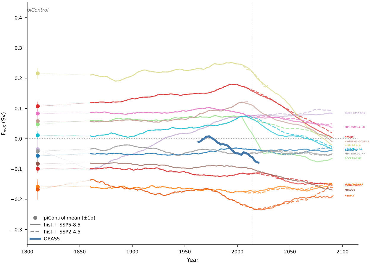
F_{ovS} trajectory: piControl \rightarrow historical \rightarrow SSP (13 CMIP6 models, n=13)
