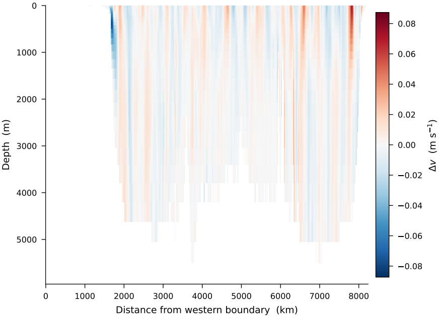
GLORYS12V1 \Delta v (late - early)
