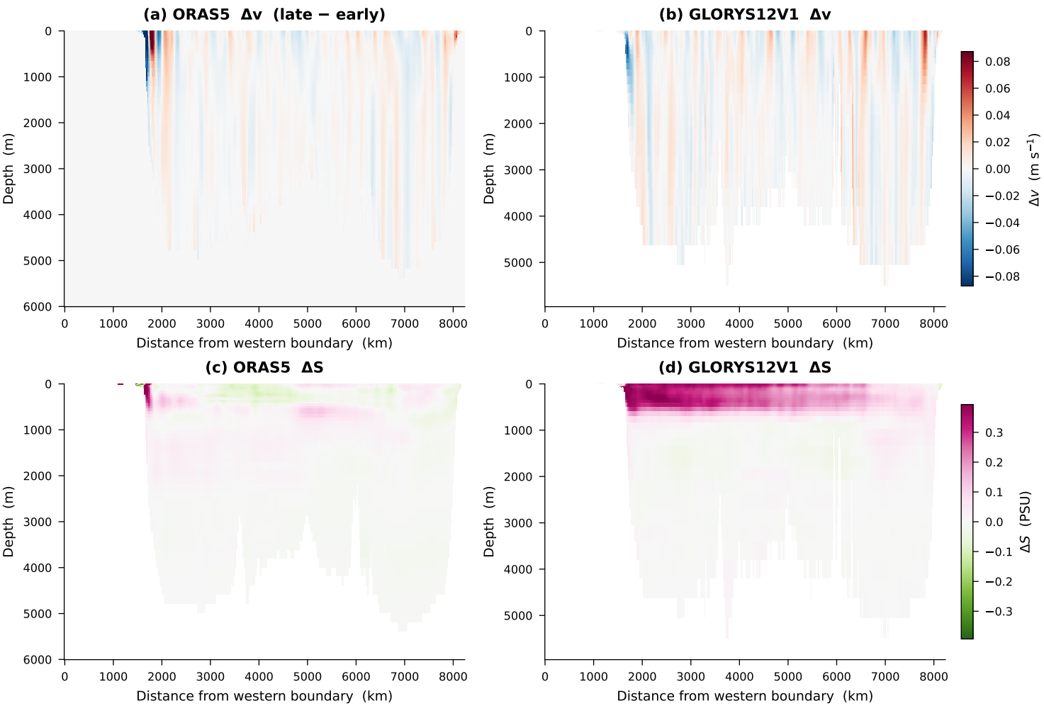
Fig. S3 — Zonal structure of \Delta v and \Delta S at 34.5°S (1993-2005 vs 2013-2025)
