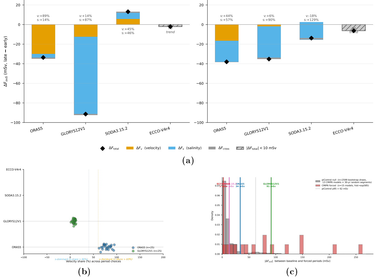
Figure 4: Robustness of the mechanism disagreement. (a) Post-Argo robustness test. Left: main windows (1993-2005 vs 2013-2025). Right: fully post-Argo windows (2006-2012 vs 2018-2024). GLORYS12V1 remains strongly salinity-dominant (+90% salinity share); ORAS5 shifts from velocity-dominant to mixed – indicating part of its signal may be an observing-system shock. (b) Sensitivity to period choice. Velocity-share ( f_v ) distributions across 25 early/late window pairs. ORAS5 and GLORYS12V1 distributions never overlap – the mechanism disagreement is robust. (c) Signal-to-noise test. Histogram of |\Delta F_{\text{ovs}}| from 2600 piControl 30-year segments (internal variability). ORAS5 (31 mSv) and GLORYS12V1 (87 mSv) exceed the 95th percentile (22 mSv), confirming their mechanism attributions are signal-dominated, not noise.
