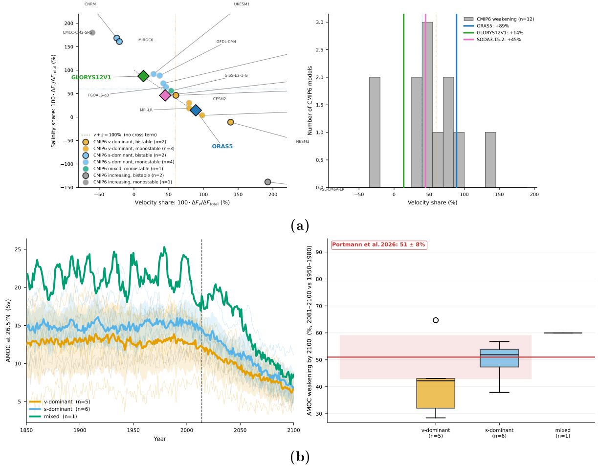
Figure 2: CMIP6 mirrors the reanalysis split and reveals a hidden 10% uncertainty in AMOC weakening. (a) Velocity-share vs salinity-share for 12 CMIP6 models with forced AMOC weakening. Symbol edge: black = bistable baseline, grey = monostable. ORAS5 (blue) and GLORYS12V1 (green) lie at opposite corners of the CMIP6 cloud. Right panel: distribution of velocity-shares, confirming the split. (b) Mechanism-conditional AMOC projections. Left: historical and future AMOC at 26.5°N for salinity-dominant (blue) and velocity-dominant (orange) models. Right: projected weakening by 2100: salinity-dominant median 52%, velocity-dominant median 42% – a \sim 10 -point gap. Red ribbon: observational constraint from Portmann et al. 9 ( 51 \pm 8\% ).
