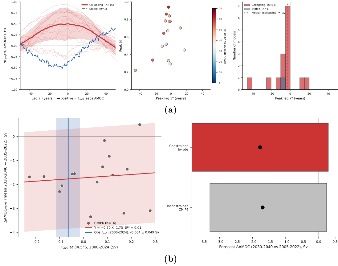
Figure 6: Supporting analyses: lead-lag relationships and emergent constraint. (a) Cross-correlation between F_{ovs} and AMOC. Left: lead-lag curves for individual CMIP6 models. Middle: per-model peak correlation lag. Right: distribution of peak lags – most models show F_{ovs} leading AMOC changes, consistent with F_{ovs} as a fingerprint. (b) Emergent constraint on F_{ovs} and future AMOC. Scatter of historical F_{ovs} (2000-2024) vs end-of-century F_{ovs} in CMIP6. The observed value ( -0.078 \pm 0.024 Sv) constrains the future F_{ovs} but does not distinguish mechanism – highlighting the need for mechanism-conditional constraints.
