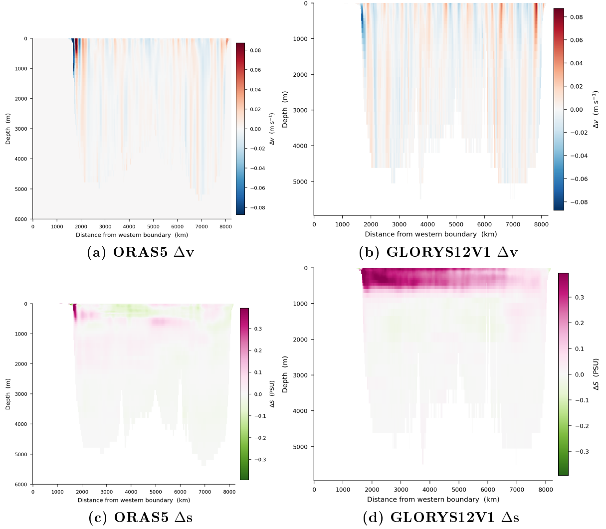
Figure 5: Zonal structure of \Delta v and \Delta S at 34.5^\circ\text{S} . ORAS5 shows large velocity changes ( \Delta v ) concentrated in the western boundary current region, consistent with a circulation-driven freshening. In contrast, GLORYS12V1 displays a basin-scale positive salinity change ( \Delta S ) in the upper 1000 m – the salt-pile-up signature predicted by active salt-advection feedback. These distinct spatial patterns provide direct observational evidence for the opposite mechanism attributions shown in Figure 1b.
