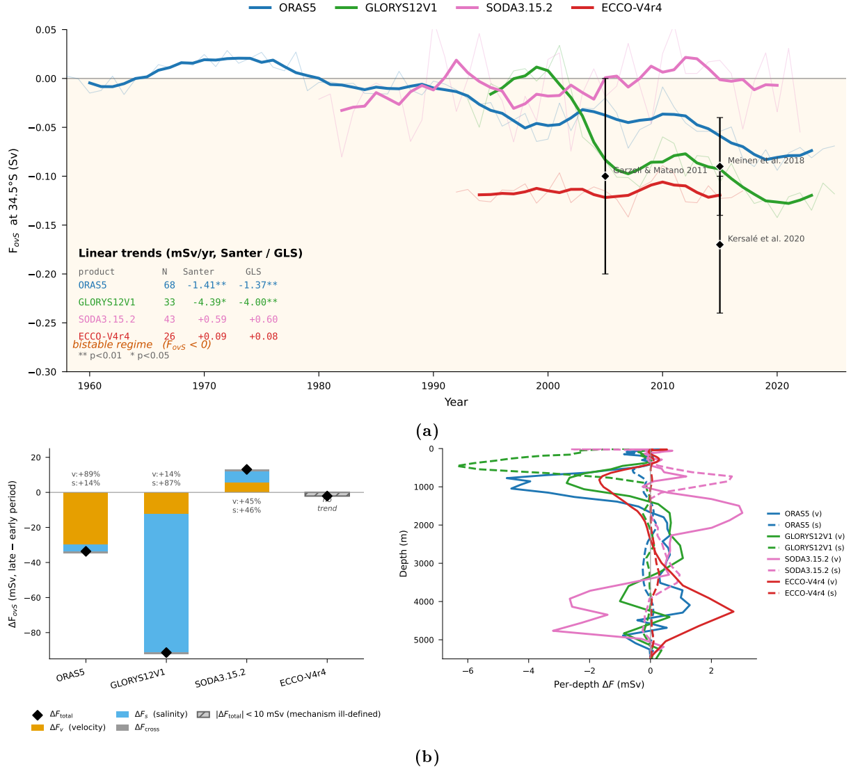
Figure 1: Atlantic bistability and opposing mechanisms for freshening. (a) Long-term F_{ovs} time series at 34.5°S. The shaded region ( F_{ovs} < 0 ) indicates the bistable regime of the salt-advection feedback, where a weakening AMOC would increase North Atlantic salinity – a positive feedback that can lead to a collapsed overturning state. Diamonds denote direct hydrography estimates. All four reanalyses have negative mean values, confirming that the Atlantic resides in the bistable regime. (b) Mechanism decomposition of the F_{ovs} change between 1993-2005 and 2013-2025. The change \Delta F_{ovs} is split into a velocity-driven part \Delta F_v (due to circulation changes only), a salinity-driven part \Delta F_s (due to salinity redistribution only), and a cross term \Delta F_{cross} (correlations). The left panel shows that ORAS5 is 89% velocity-driven (circulation change dominates), whereas GLORYS12V1 is 87% salinity-driven – the direct fingerprint of active salt-advection feedback. The right panel displays vertical profiles of the integrands, revealing that the opposite attributions originate from depth-dependent differences in velocity and salinity anomalies. These opposing mechanisms imply fundamentally different future AMOC trajectories, as quantified in Figure 2.
