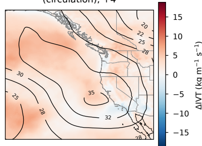
(f) Dynamic + \Delta z_{500} (circulation), +4
