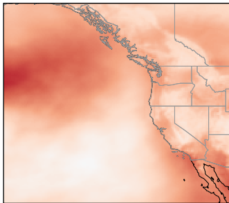
(e) Thermodynamic (moisture/CC), +7
